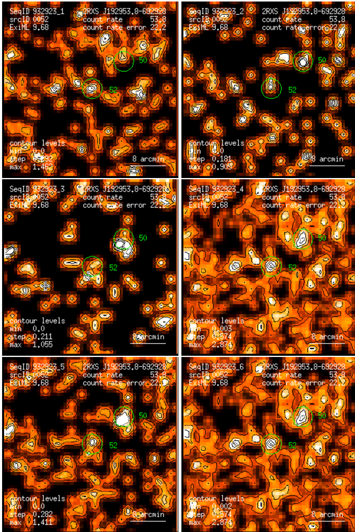
Figure 52: RASS 932923: detection 0052: band rate images, Gaussian filter: (1) PSPC channels 11 – 41, (2) 52 – 90, (3) 91 – 201, (4) 11 – 235, (5) 52 – 201, (6) 11 – 201. Broad band rates in counts/ks. Band rate contour levels in counts/ks/arcmin 2 .
