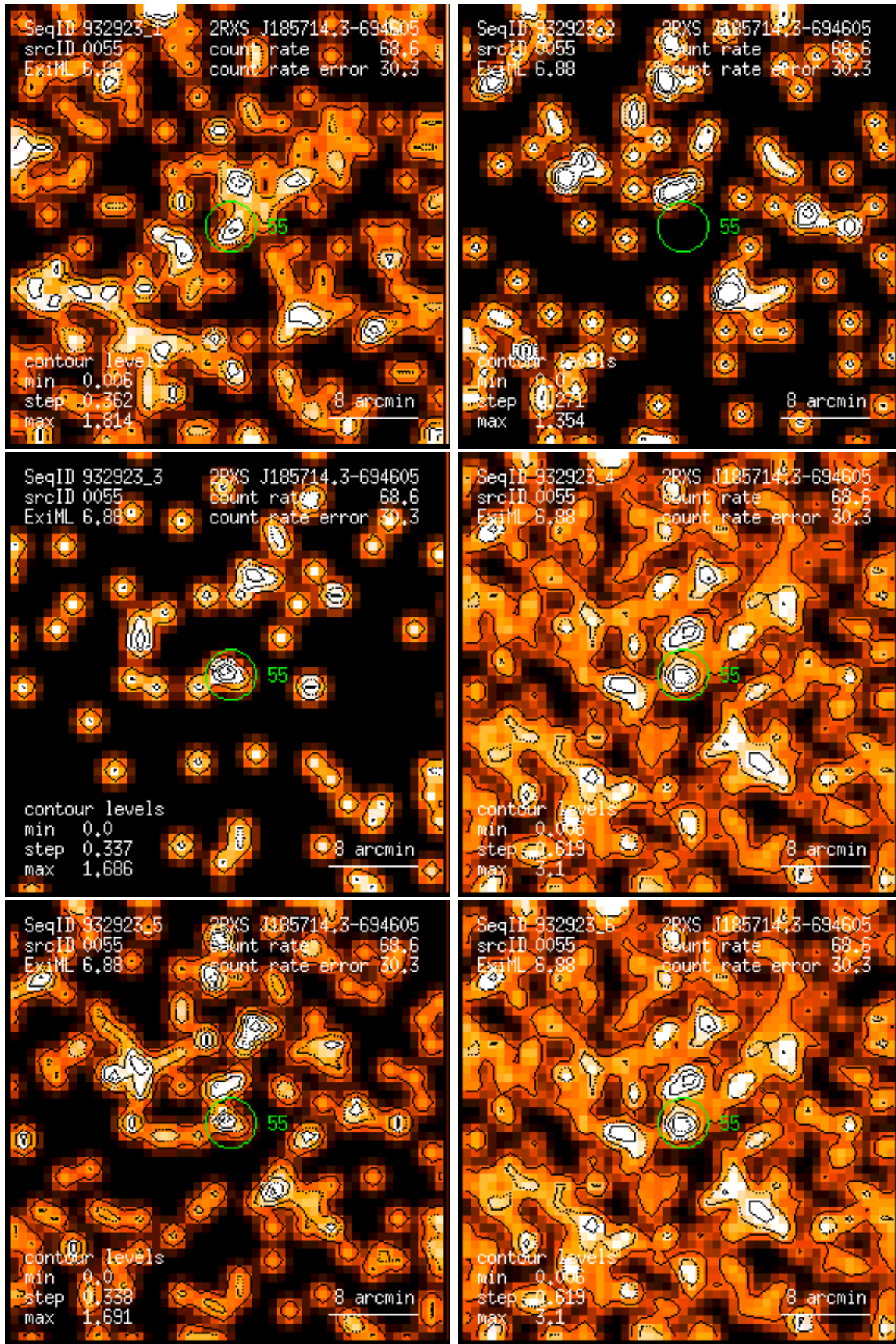
Figure 55: RASS 932923: detection 0055: band rate images, Gaussian filter: (1) PSPC channels 11 – 41, (2) 52 – 90, (3) 91 – 201, (4) 11 – 235, (5) 52 – 201, (6) 11 – 201. Broad band rates in counts/ks. Band rate contour levels in counts/ks/arcmin 2 .
