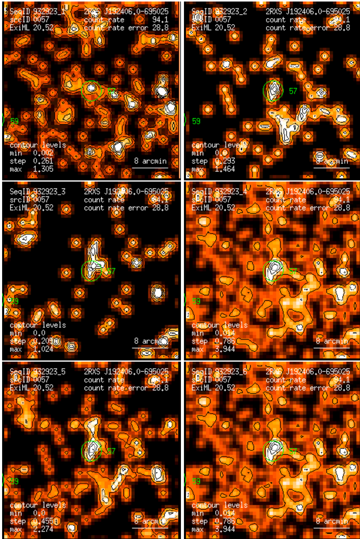
Figure 57: RASS 932923: detection 0057: band rate images, Gaussian filter: (1) PSPC channels 11 – 41, (2) 52 – 90, (3) 91 – 201, (4) 11 – 235, (5) 52 – 201, (6) 11 – 201. Broad band rates in counts/ks. Band rate contour levels in counts/ks/arcmin 2 .
