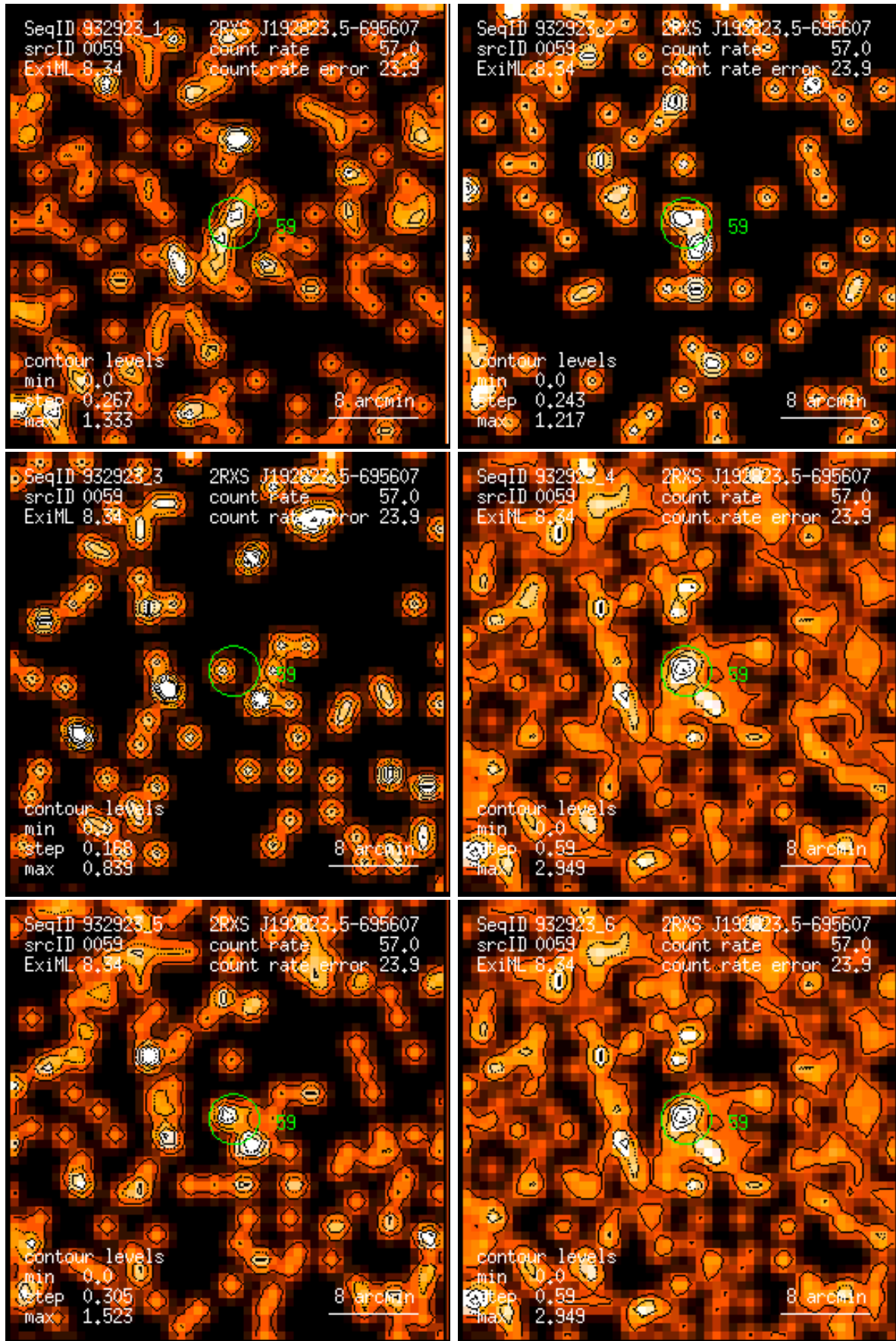
Figure 59: RASS 932923: detection 0059: band rate images, Gaussian filter: (1) PSPC channels 11 – 41, (2) 52 – 90, (3) 91 – 201, (4) 11 – 235, (5) 52 – 201, (6) 11 – 201. Broad band rates in counts/ks. Band rate contour levels in counts/ks/arcmin 2 .
