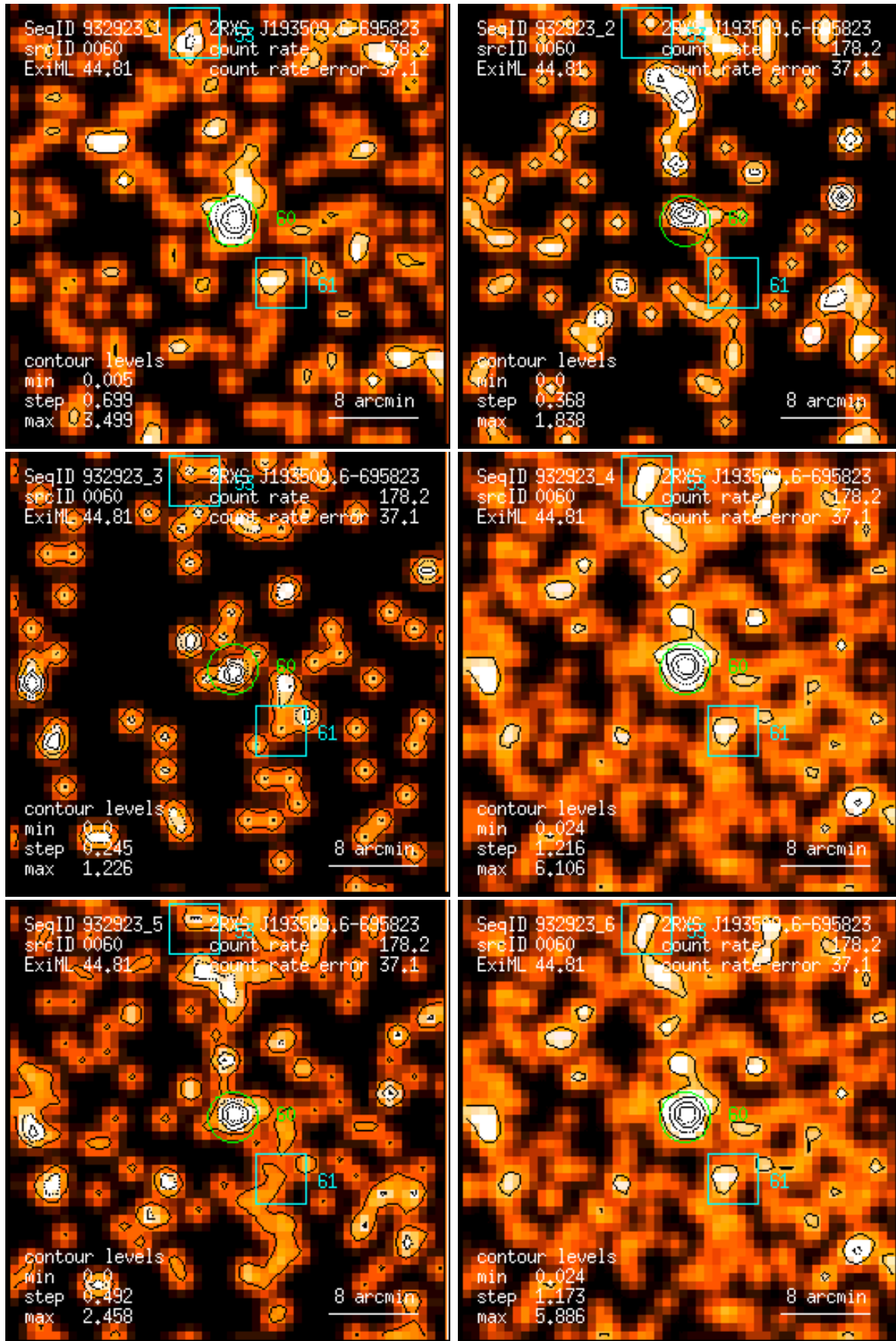
Figure 60: RASS 932923: detection 0060: band rate images, Gaussian filter: (1) PSPC channels 11 – 41, (2) 52 – 90, (3) 91 – 201, (4) 11 – 235, (5) 52 – 201, (6) 11 – 201. Broad band rates in counts/ks. Band rate contour levels in counts/ks/arcmin 2 .
