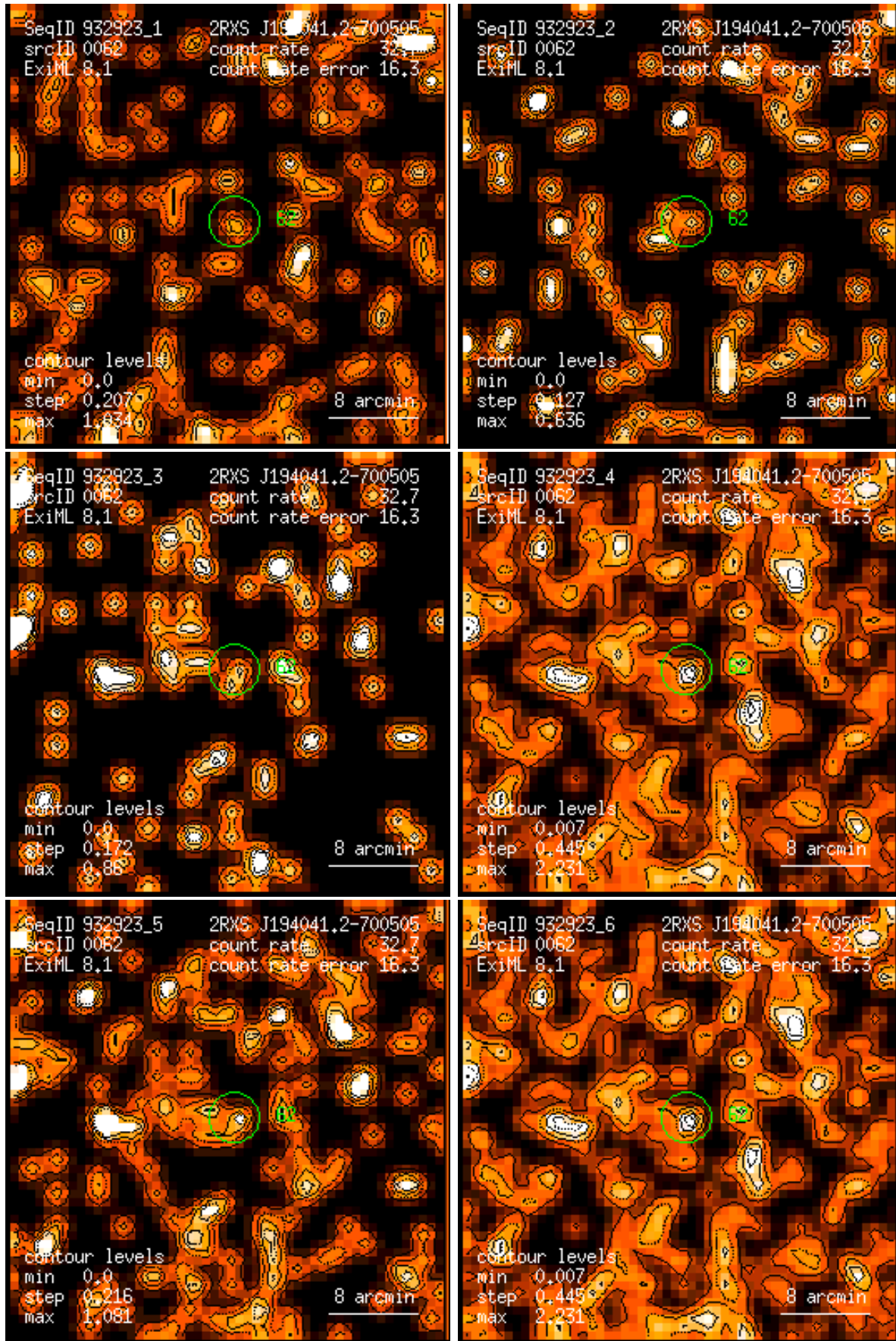
Figure 62: RASS 932923: detection 0062: band rate images, Gaussian filter: (1) PSPC channels 11 – 41, (2) 52 – 90, (3) 91 – 201, (4) 11 – 235, (5) 52 – 201, (6) 11 – 201. Broad band rates in counts/ks. Band rate contour levels in counts/ks/arcmin 2 .
