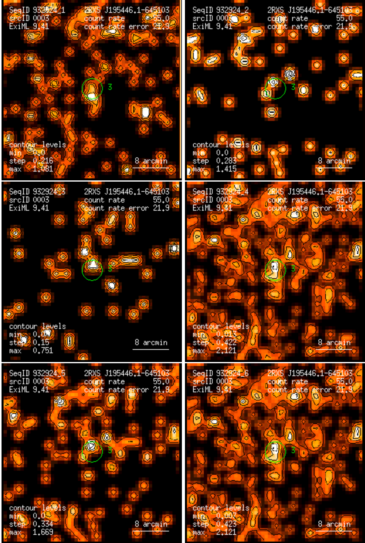
Figure 3: RASS 932924: detection 0003: band rate images, Gaussian filter: (1) PSPC channels 11 – 41, (2) 52 – 90, (3) 91 – 201, (4) 11 – 235, (5) 52 – 201, (6) 11 – 201. Broad band rates in counts/ks. Band rate contour levels in counts/ks/arcmin 2 .
