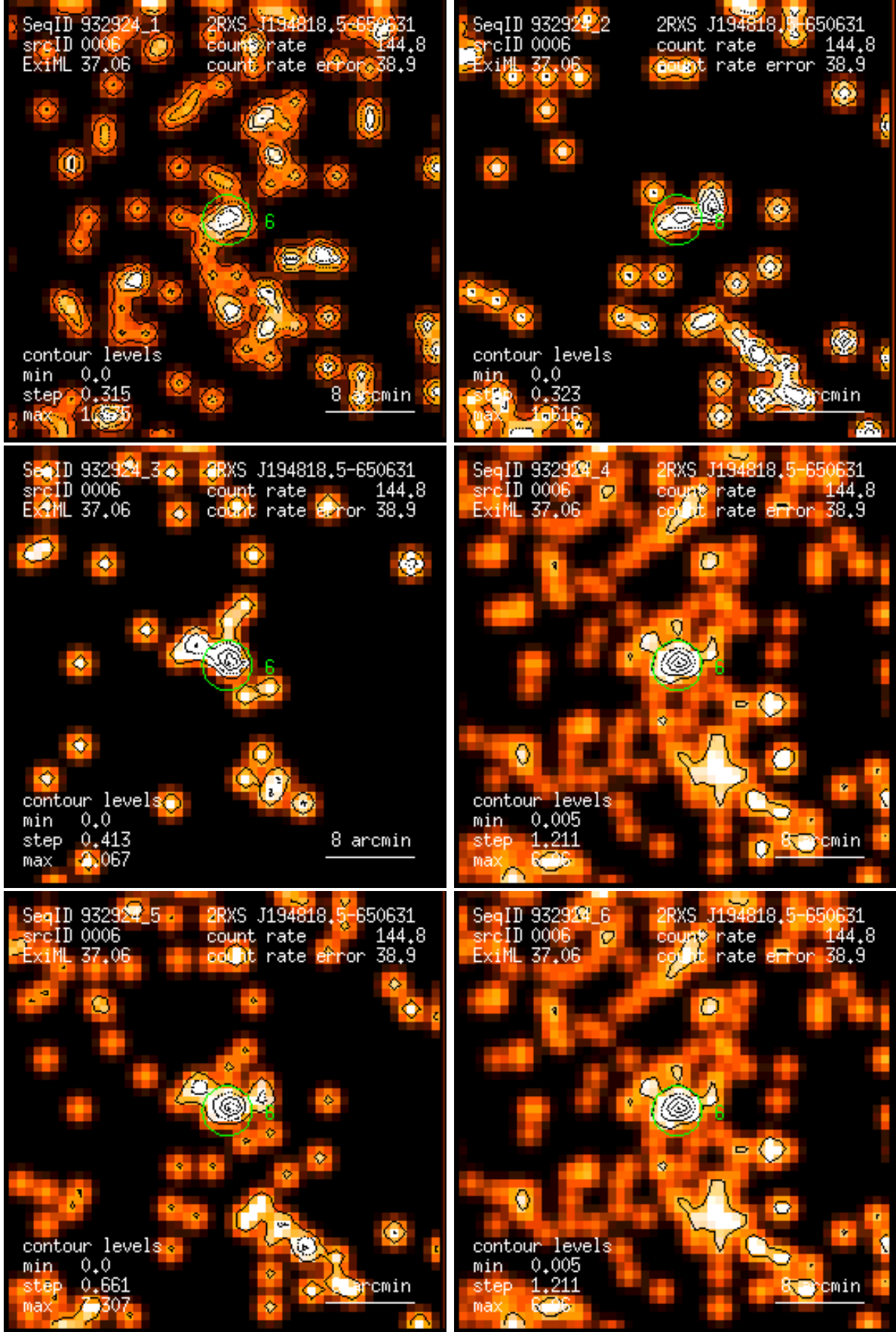
Figure 6: RASS 932924: detection 0006: band rate images, Gaussian filter: (1) PSPC channels 11 – 41, (2) 52 – 90, (3) 91 – 201, (4) 11 – 235, (5) 52 – 201, (6) 11 – 201. Broad band rates in counts/ks. Band rate contour levels in counts/ks/arcmin 2 .
