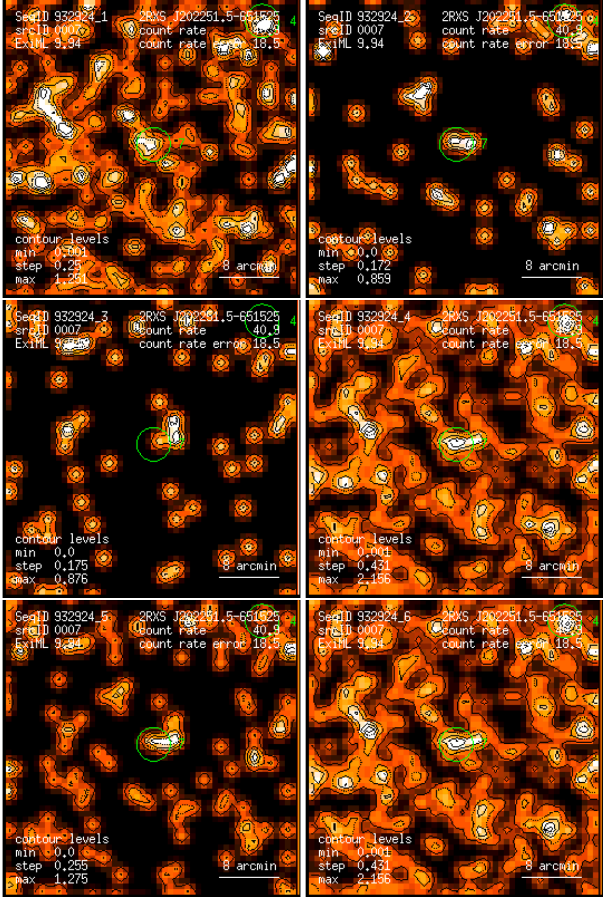
Figure 7: RASS 932924: detection 0007: band rate images, Gaussian filter: (1) PSPC channels 11 – 41, (2) 52 – 90, (3) 91 – 201, (4) 11 – 235, (5) 52 – 201, (6) 11 – 201. Broad band rates in counts/ks. Band rate contour levels in counts/ks/arcmin 2 .
