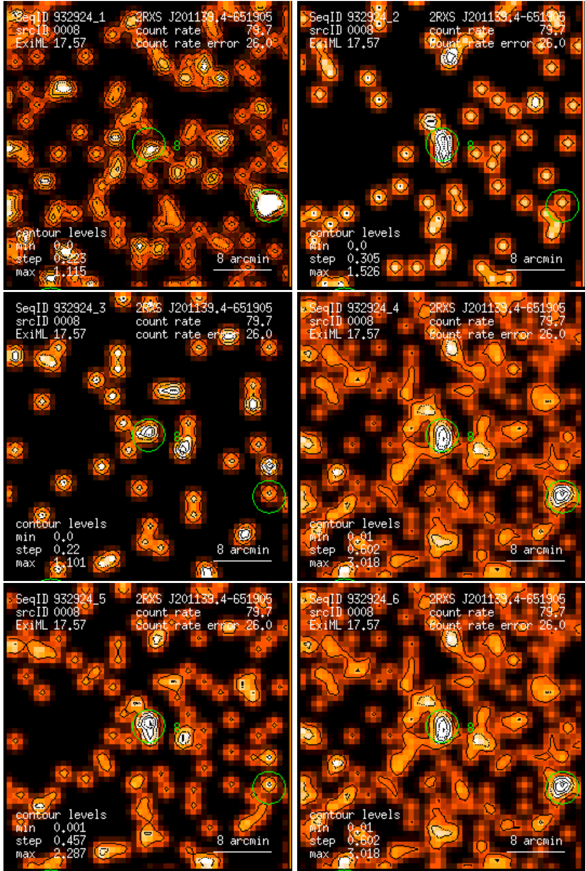
Figure 8: RASS 932924: detection 0008: band rate images, Gaussian filter: (1) PSPC channels 11 – 41, (2) 52 – 90, (3) 91 – 201, (4) 11 – 235, (5) 52 – 201, (6) 11 – 201. Broad band rates in counts/ks. Band rate contour levels in counts/ks/arcmin 2 .
