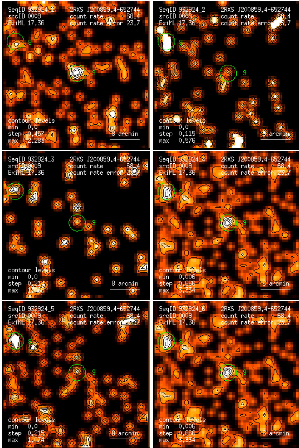
Figure 9: RASS 932924: detection 0009: band rate images, Gaussian filter: (1) PSPC channels 11 – 41, (2) 52 – 90, (3) 91 – 201, (4) 11 – 235, (5) 52 – 201, (6) 11 – 201. Broad band rates in counts/ks. Band rate contour levels in counts/ks/arcmin 2 .
