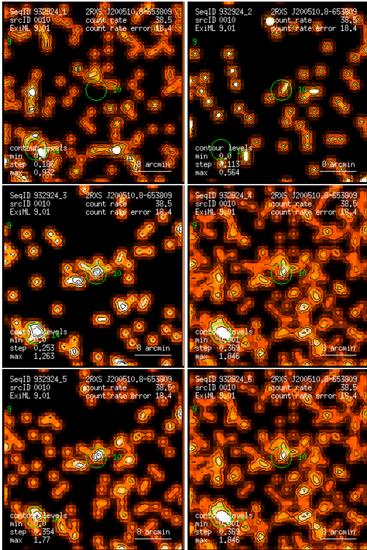
Figure 10: RASS 932924: detection 0010: band rate images, Gaussian filter: (1) PSPC channels 11 – 41, (2) 52 – 90, (3) 91 – 201, (4) 11 – 235, (5) 52 – 201, (6) 11 – 201. Broad band rates in counts/ks. Band rate contour levels in counts/ks/arcmin 2 .
