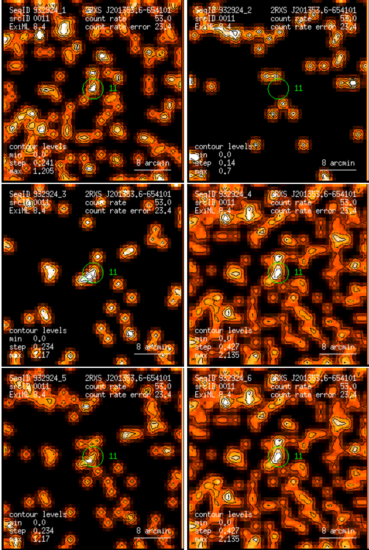
Figure 11: RASS 932924: detection 0011: band rate images, Gaussian filter: (1) PSPC channels 11 – 41, (2) 52 – 90, (3) 91 – 201, (4) 11 – 235, (5) 52 – 201, (6) 11 – 201. Broad band rates in counts/ks. Band rate contour levels in counts/ks/arcmin 2 .
