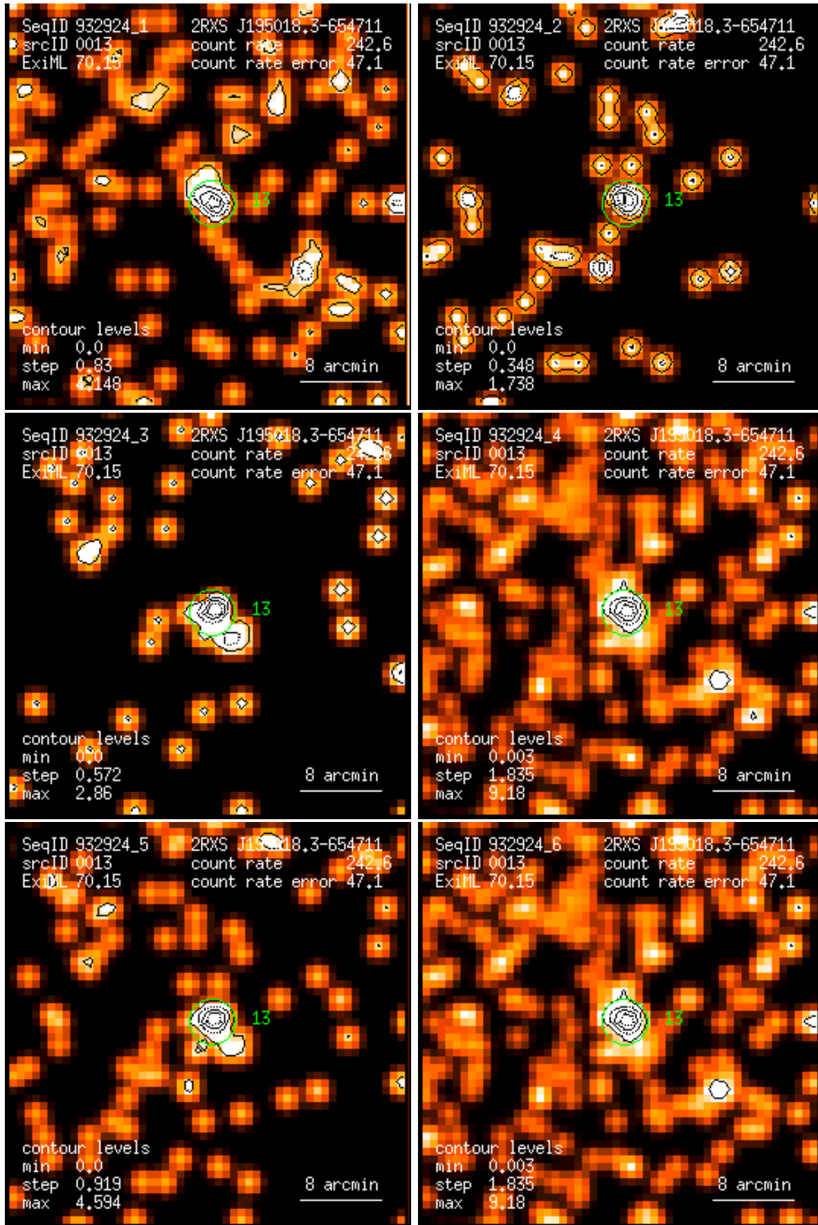
Figure 13: RASS 932924: detection 0013: band rate images, Gaussian filter: (1) PSPC channels 11 – 41, (2) 52 – 90, (3) 91 – 201, (4) 11 – 235, (5) 52 – 201, (6) 11 – 201. Broad band rates in counts/ks. Band rate contour levels in counts/ks/arcmin 2 .
