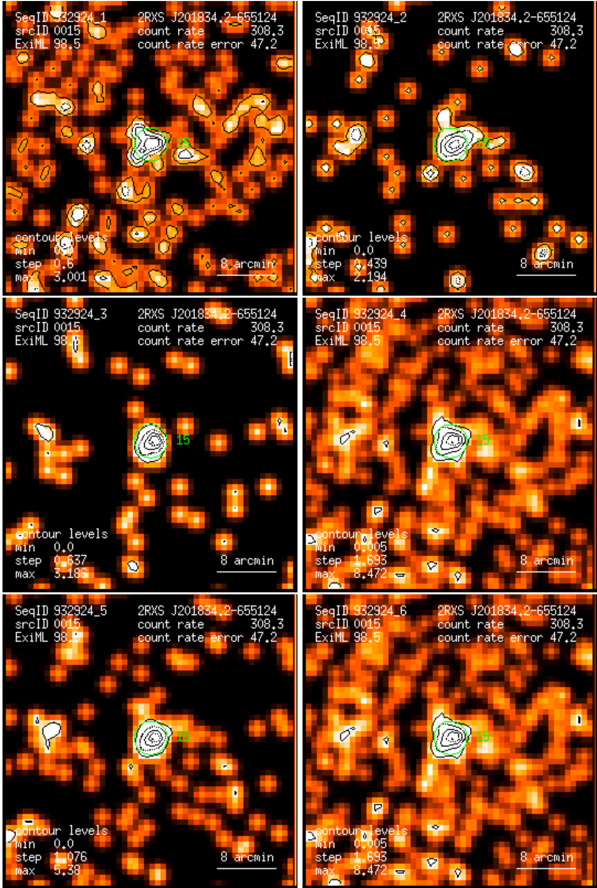
Figure 15: RASS 932924: detection 0015: band rate images, Gaussian filter: (1) PSPC channels 11 – 41, (2) 52 – 90, (3) 91 – 201, (4) 11 – 235, (5) 52 – 201, (6) 11 – 201. Broad band rates in counts/ks. Band rate contour levels in counts/ks/arcmin 2 .
