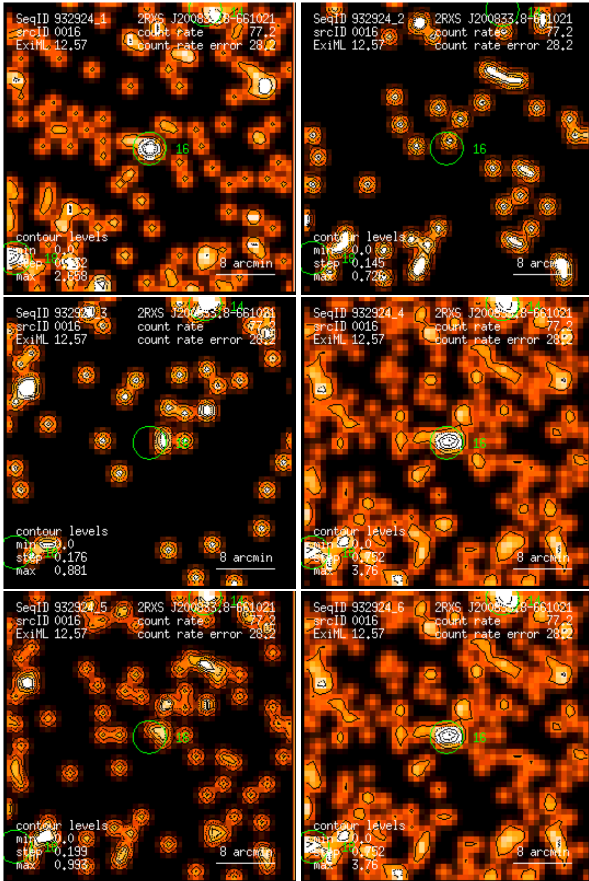
Figure 16: RASS 932924: detection 0016: band rate images, Gaussian filter: (1) PSPC channels 11 – 41, (2) 52 – 90, (3) 91 – 201, (4) 11 – 235, (5) 52 – 201, (6) 11 – 201. Broad band rates in counts/ks. Band rate contour levels in counts/ks/arcmin 2 .
