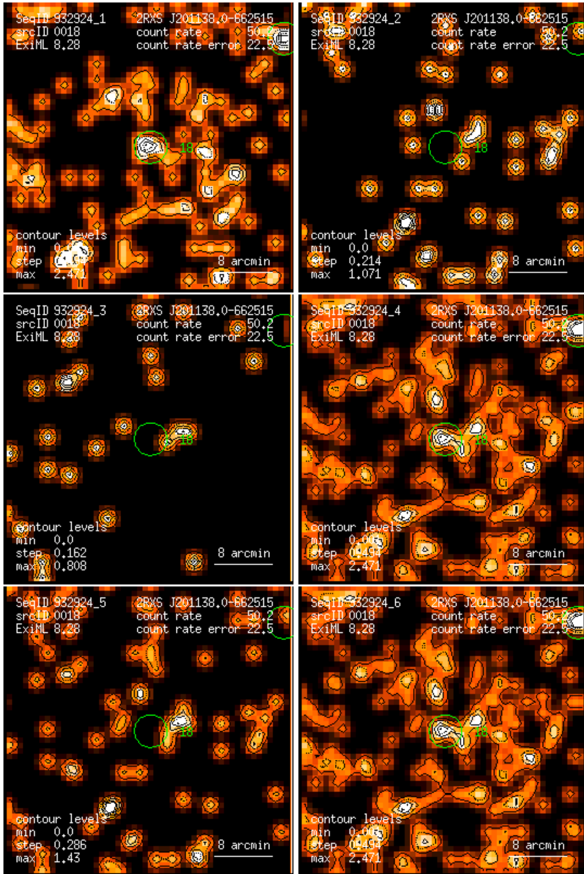
Figure 18: RASS 932924: detection 0018: band rate images, Gaussian filter: (1) PSPC channels 11 – 41, (2) 52 – 90, (3) 91 – 201, (4) 11 – 235, (5) 52 – 201, (6) 11 – 201. Broad band rates in counts/ks. Band rate contour levels in counts/ks/arcmin 2 .
