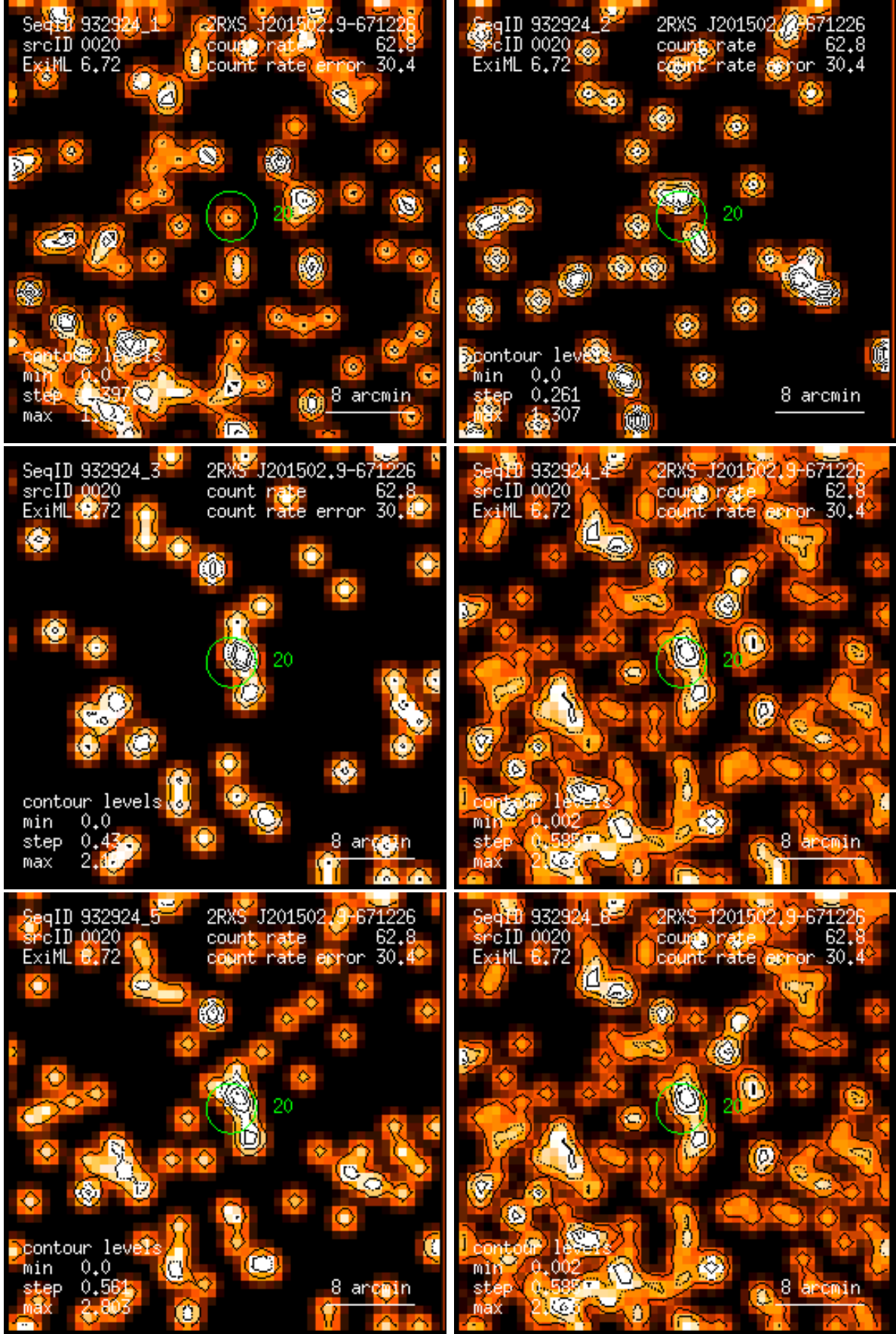
Figure 20: RASS 932924: detection 0020: band rate images, Gaussian filter: (1) PSPC channels 11 – 41, (2) 52 – 90, (3) 91 – 201, (4) 11 – 235, (5) 52 – 201, (6) 11 – 201. Broad band rates in counts/ks. Band rate contour levels in counts/ks/arcmin 2 .
