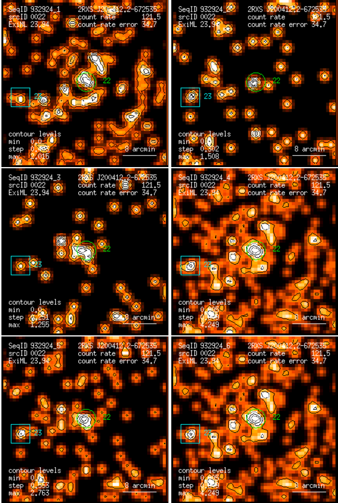
Figure 22: RASS 932924: detection 0022: band rate images, Gaussian filter: (1) PSPC channels 11 – 41, (2) 52 – 90, (3) 91 – 201, (4) 11 – 235, (5) 52 – 201, (6) 11 – 201. Broad band rates in counts/ks. Band rate contour levels in counts/ks/arcmin 2 .
