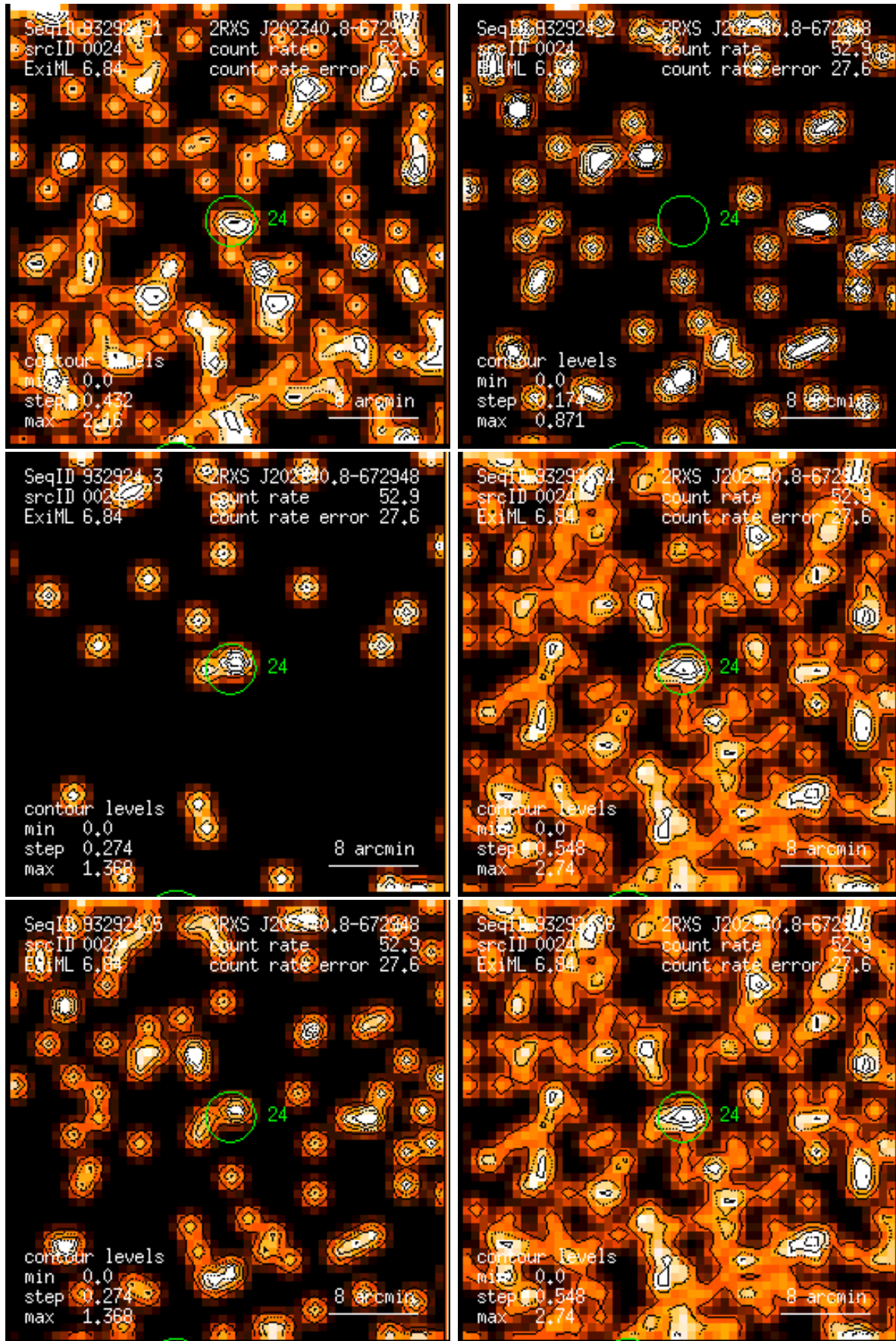
Figure 24: RASS 932924: detection 0024: band rate images, Gaussian filter: (1) PSPC channels 11 – 41, (2) 52 – 90, (3) 91 – 201, (4) 11 – 235, (5) 52 – 201, (6) 11 – 201. Broad band rates in counts/ks. Band rate contour levels in counts/ks/arcmin 2 .
