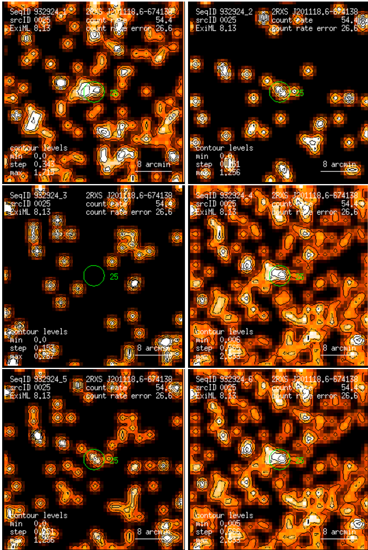
Figure 25: RASS 932924: detection 0025: band rate images, Gaussian filter: (1) PSPC channels 11 – 41, (2) 52 – 90, (3) 91 – 201, (4) 11 – 235, (5) 52 – 201, (6) 11 – 201. Broad band rates in counts/ks. Band rate contour levels in counts/ks/arcmin 2 .
