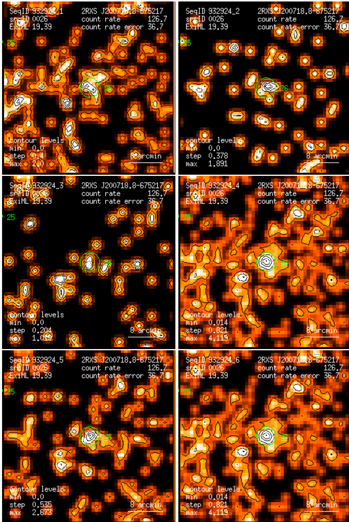
Figure 26: RASS 932924: detection 0026: band rate images, Gaussian filter: (1) PSPC channels 11 – 41, (2) 52 – 90, (3) 91 – 201, (4) 11 – 235, (5) 52 – 201, (6) 11 – 201. Broad band rates in counts/ks. Band rate contour levels in counts/ks/arcmin 2 .
