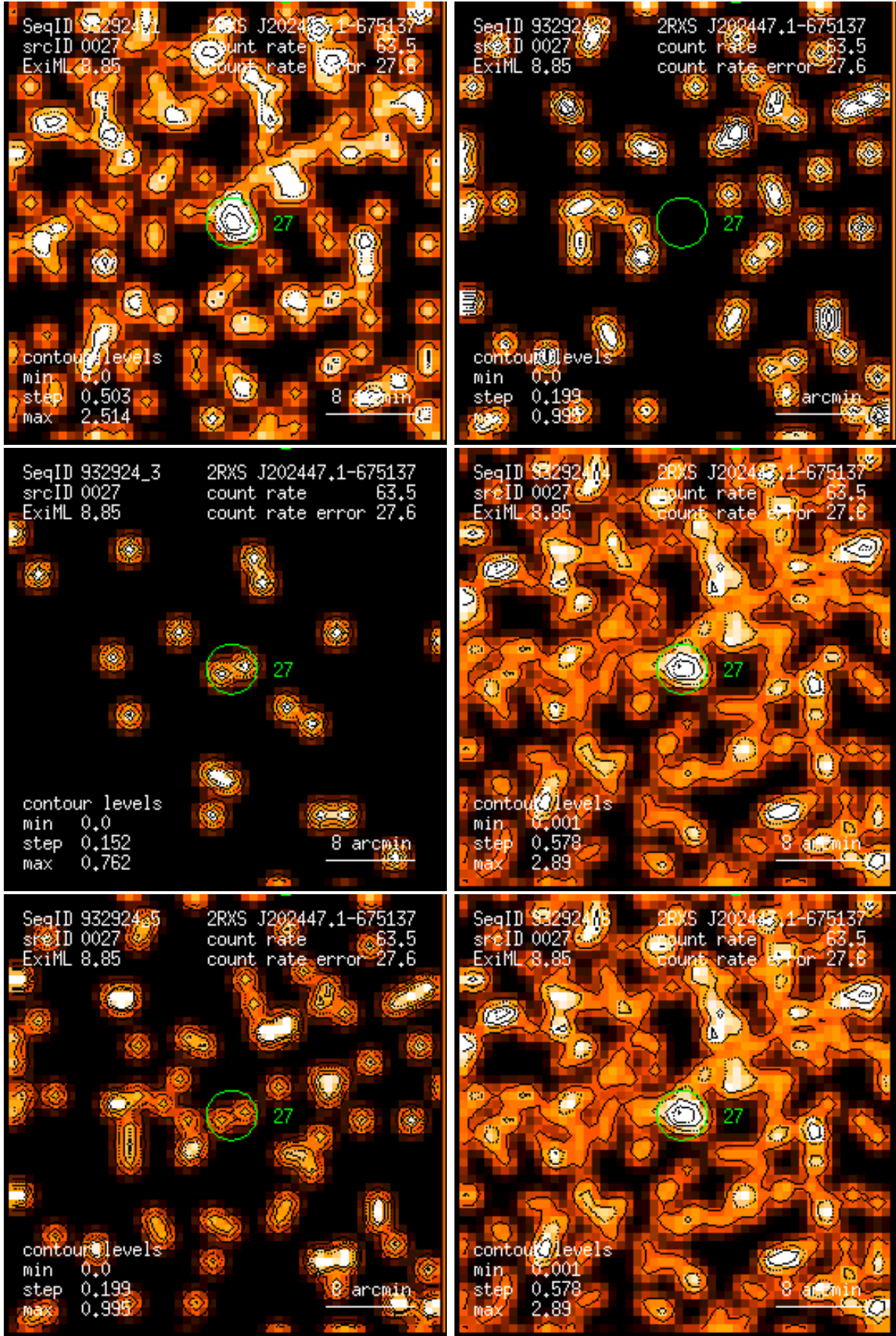
Figure 27: RASS 932924: detection 0027: band rate images, Gaussian filter: (1) PSPC channels 11 – 41, (2) 52 – 90, (3) 91 – 201, (4) 11 – 235, (5) 52 – 201, (6) 11 – 201. Broad band rates in counts/ks. Band rate contour levels in counts/ks/arcmin 2 .
