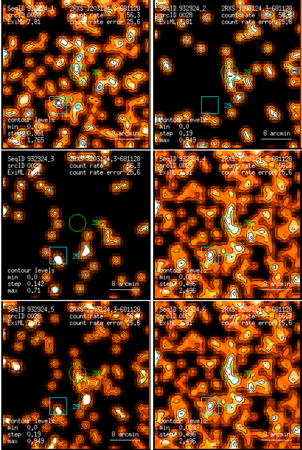
Figure 28: RASS 932924: detection 0028: band rate images, Gaussian filter: (1) PSPC channels 11 – 41, (2) 52 – 90, (3) 91 – 201, (4) 11 – 235, (5) 52 – 201, (6) 11 – 201. Broad band rates in counts/ks. Band rate contour levels in counts/ks/arcmin 2 .
