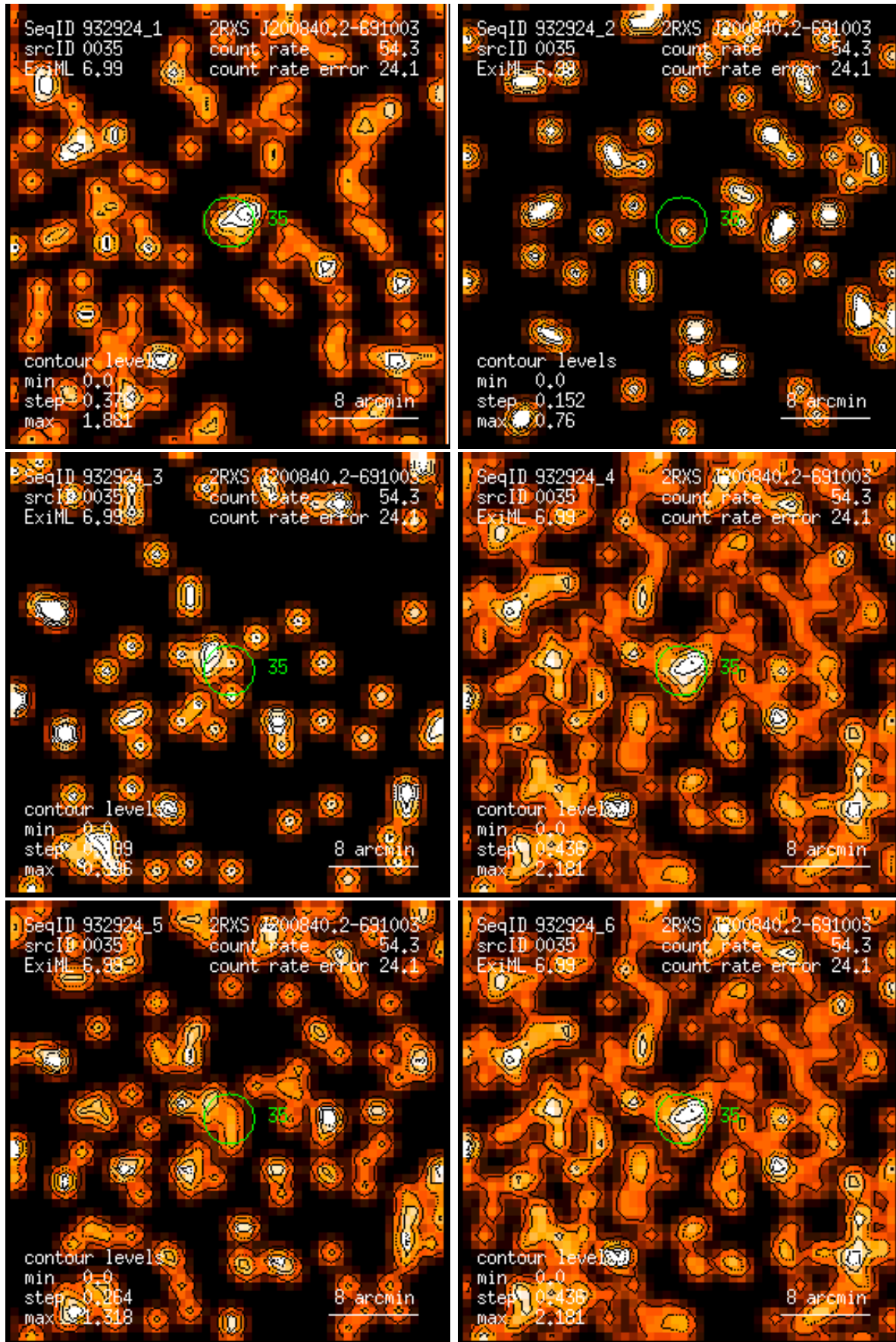
Figure 35: RASS 932924: detection 0035: band rate images, Gaussian filter: (1) PSPC channels 11 – 41, (2) 52 – 90, (3) 91 – 201, (4) 11 – 235, (5) 52 – 201, (6) 11 – 201. Broad band rates in counts/ks. Band rate contour levels in counts/ks/arcmin 2 .
