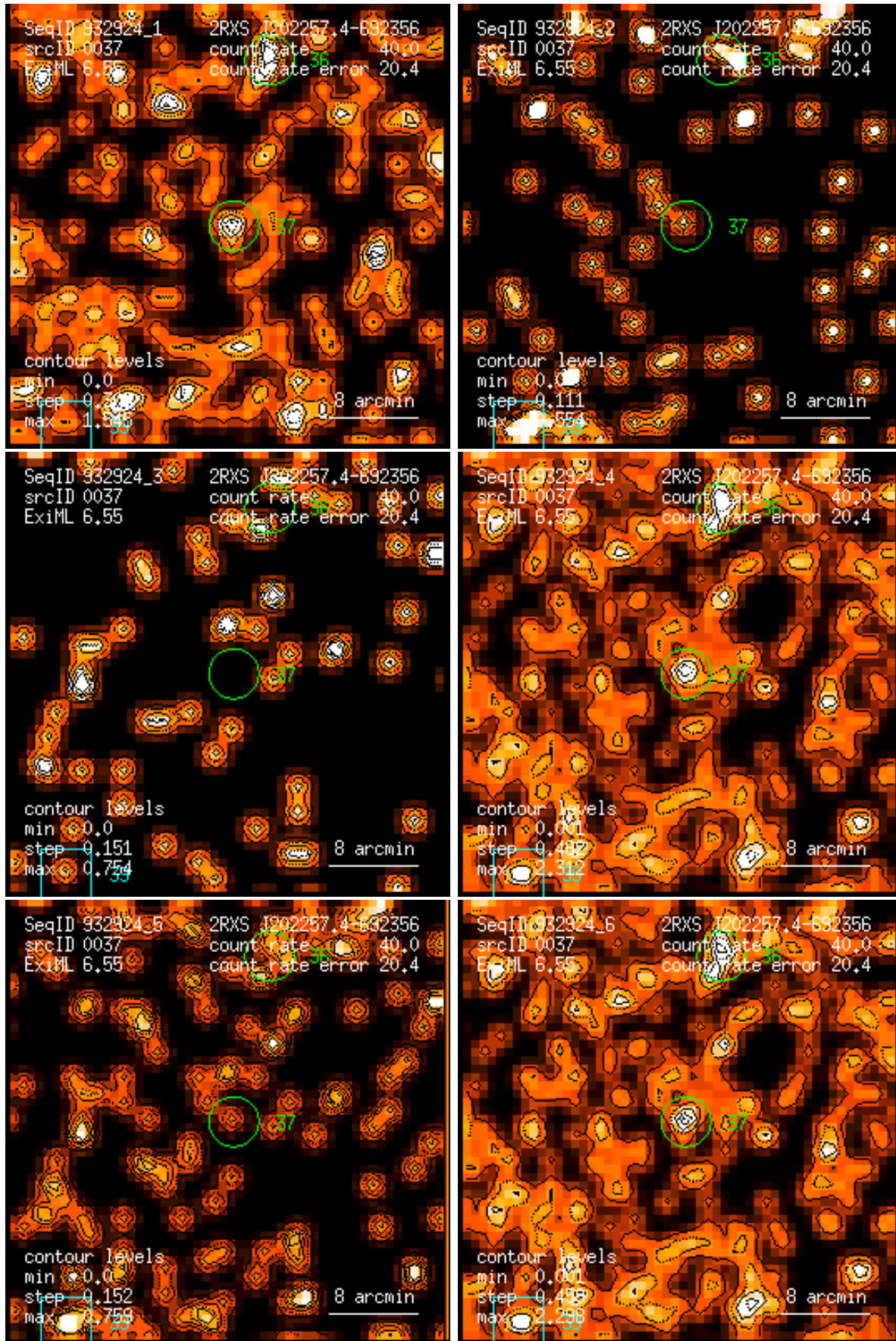
Figure 37: RASS 932924: detection 0037: band rate images, Gaussian filter: (1) PSPC channels 11 – 41, (2) 52 – 90, (3) 91 – 201, (4) 11 – 235, (5) 52 – 201, (6) 11 – 201. Broad band rates in counts/ks. Band rate contour levels in counts/ks/arcmin 2 .
