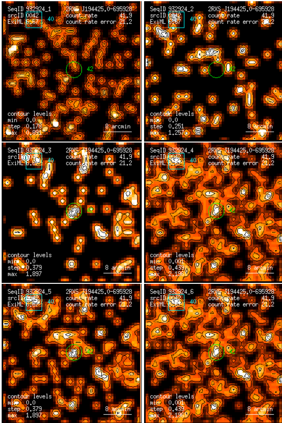
Figure 42: RASS 932924: detection 0042: band rate images, Gaussian filter: (1) PSPC channels 11 – 41, (2) 52 – 90, (3) 91 – 201, (4) 11 – 235, (5) 52 – 201, (6) 11 – 201. Broad band rates in counts/ks. Band rate contour levels in counts/ks/arcmin 2 .
