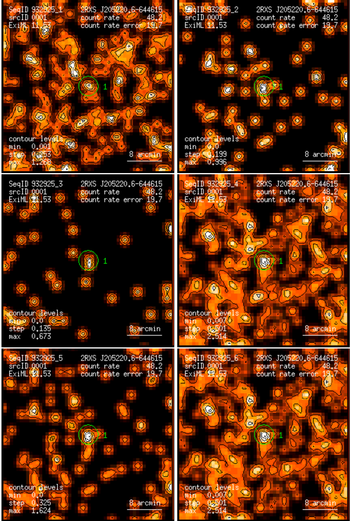
Figure 1: RASS 932925: detection 0001: band rate images, Gaussian filter: (1) PSPC channels 11 – 41, (2) 52 – 90, (3) 91 – 201, (4) 11 – 235, (5) 52 – 201, (6) 11 – 201. Broad band rates in counts/ks. Band rate contour levels in counts/ks/arcmin 2 .
