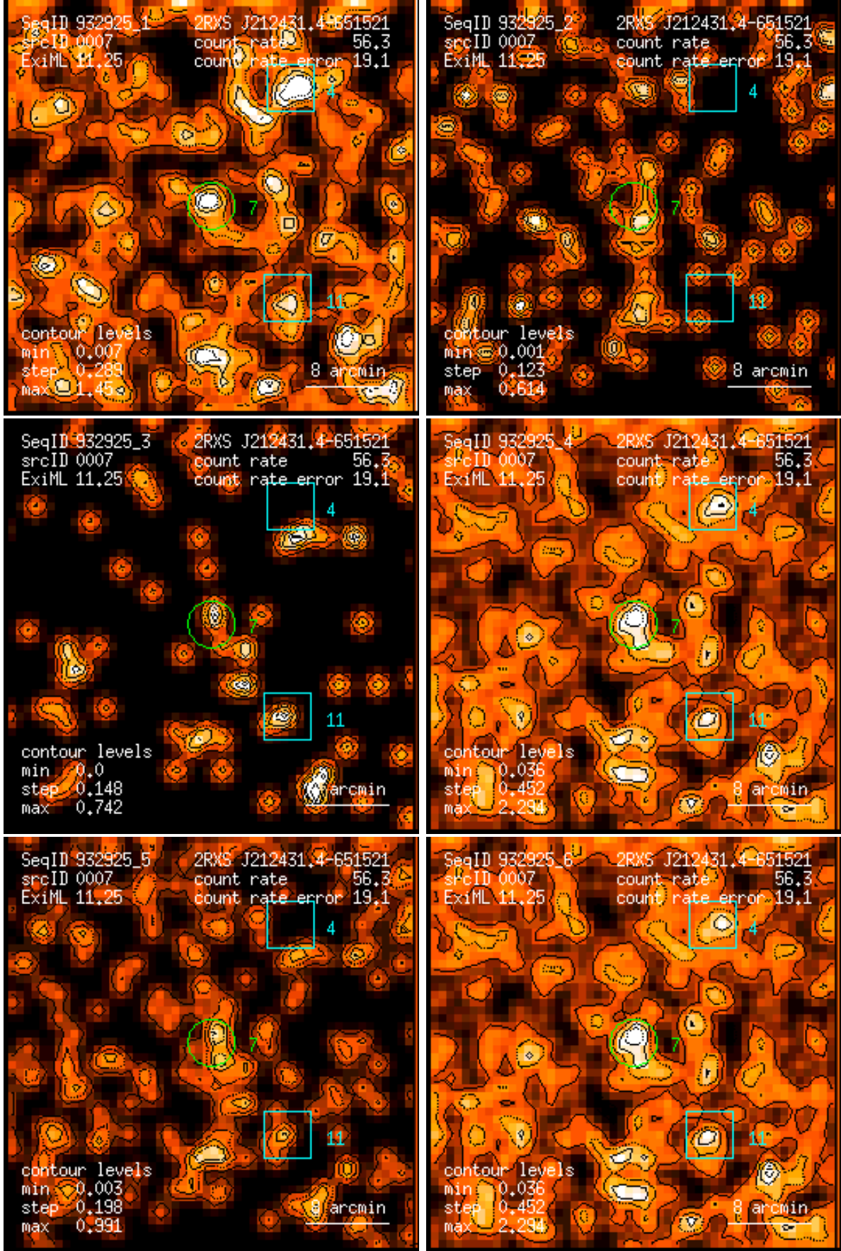
Figure 7: RASS 932925: detection 0007: band rate images, Gaussian filter: (1) PSPC channels 11 – 41, (2) 52 – 90, (3) 91 – 201, (4) 11 – 235, (5) 52 – 201, (6) 11 – 201. Broad band rates in counts/ks. Band rate contour levels in counts/ks/arcmin 2 .
