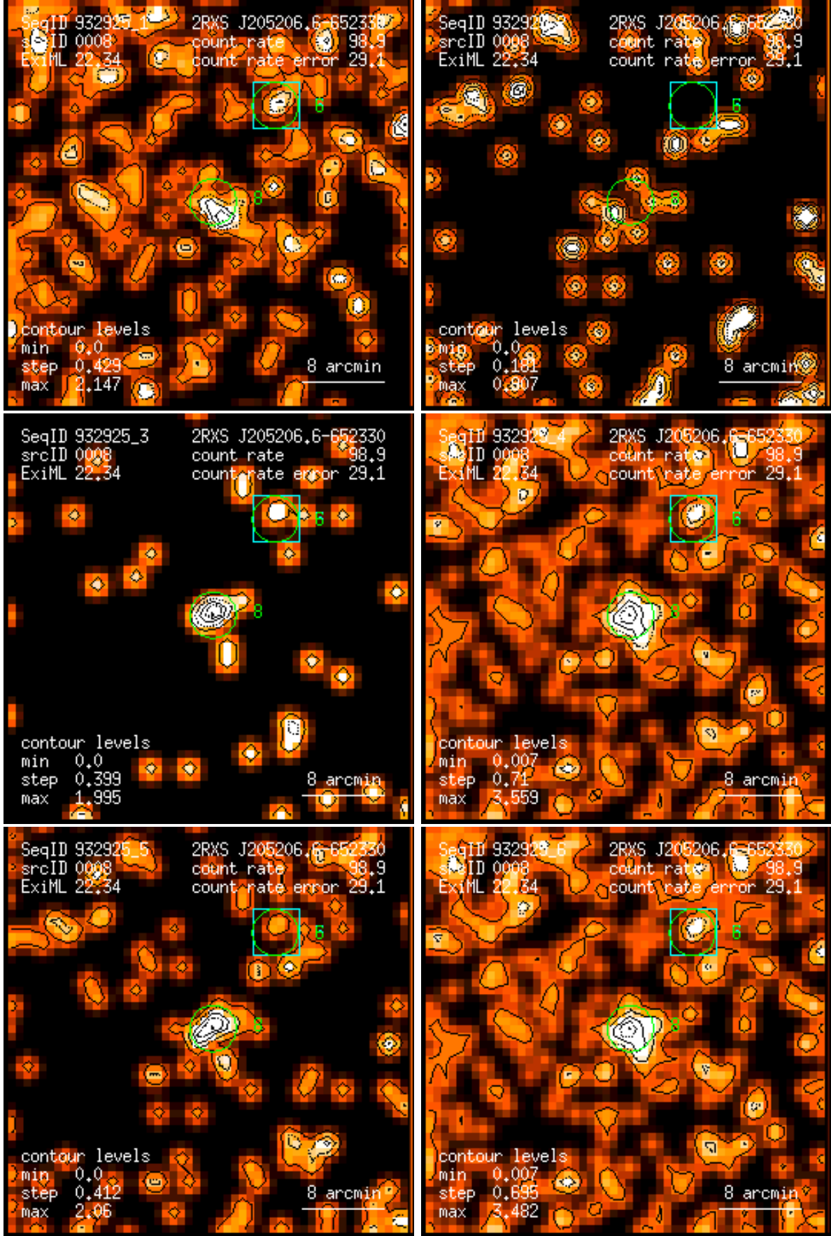
Figure 8: RASS 932925: detection 0008: band rate images, Gaussian filter: (1) PSPC channels 11 – 41, (2) 52 – 90, (3) 91 – 201, (4) 11 – 235, (5) 52 – 201, (6) 11 – 201. Broad band rates in counts/ks. Band rate contour levels in counts/ks/arcmin 2 .
