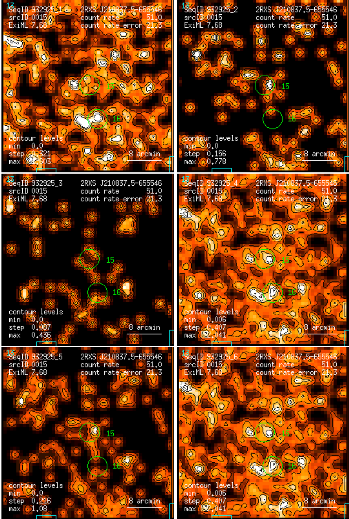
Figure 15: RASS 932925: detection 0015: band rate images, Gaussian filter: (1) PSPC channels 11 – 41, (2) 52 – 90, (3) 91 – 201, (4) 11 – 235, (5) 52 – 201, (6) 11 – 201. Broad band rates in counts/ks. Band rate contour levels in counts/ks/arcmin 2 .
