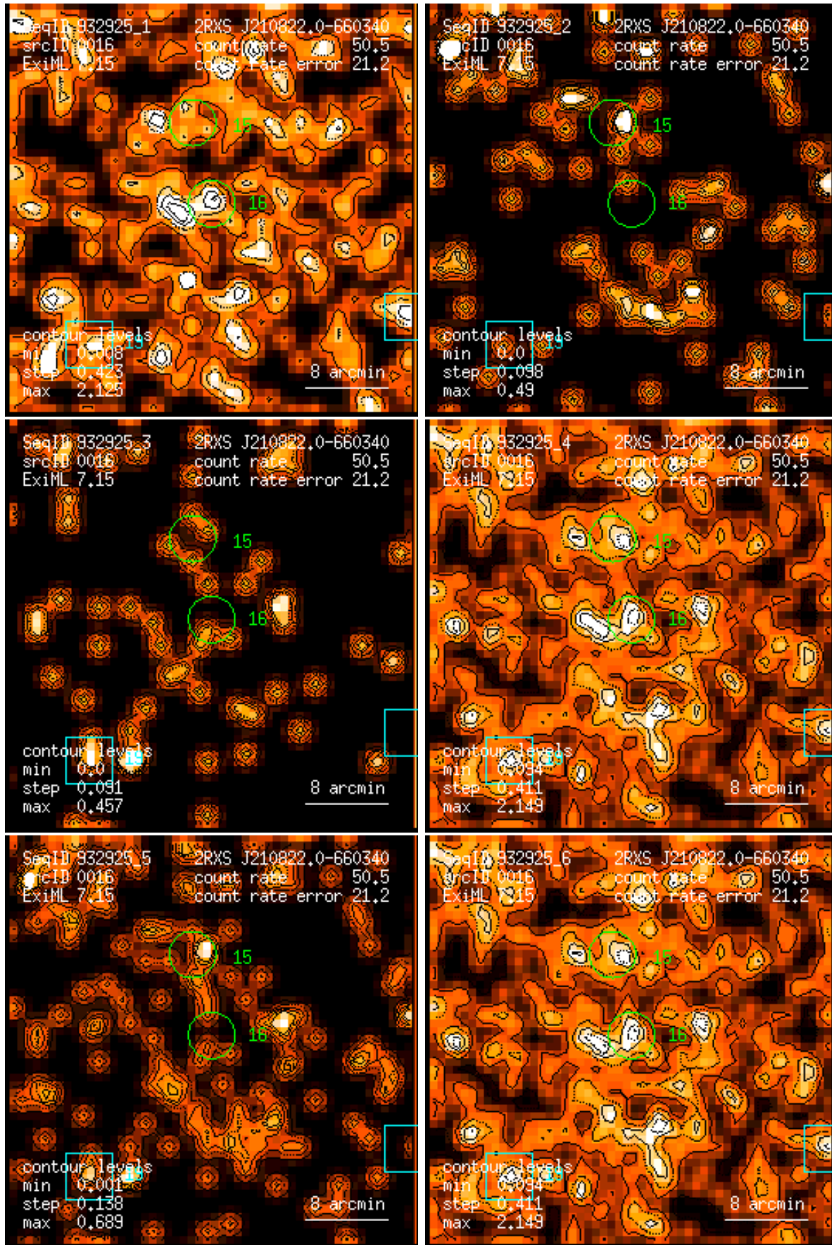
Figure 16: RASS 932925: detection 0016: band rate images, Gaussian filter: (1) PSPC channels 11 – 41, (2) 52 – 90, (3) 91 – 201, (4) 11 – 235, (5) 52 – 201, (6) 11 – 201. Broad band rates in counts/ks. Band rate contour levels in counts/ks/arcmin 2 .
