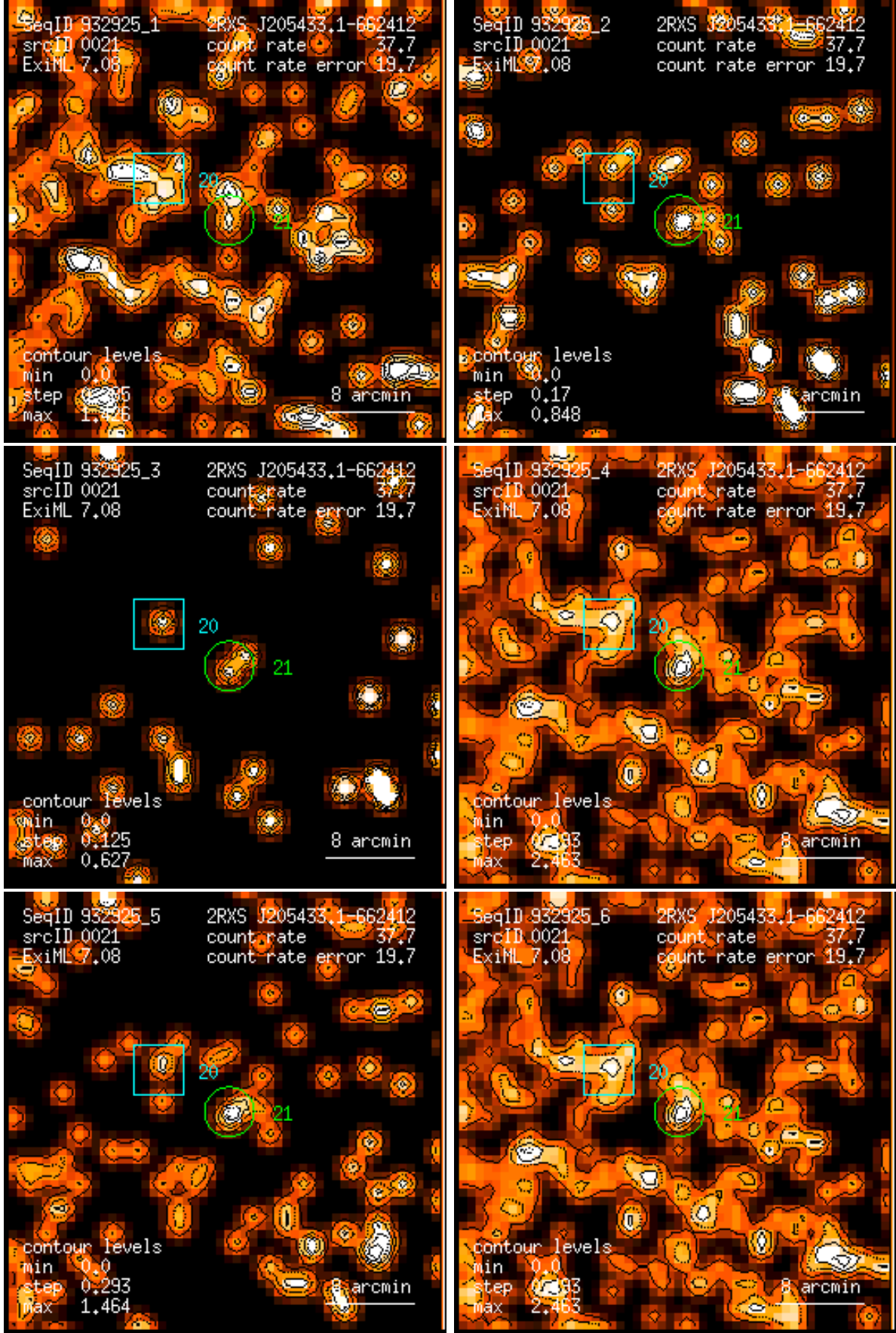
Figure 21: RASS 932925: detection 0021: band rate images, Gaussian filter: (1) PSPC channels 11 – 41, (2) 52 – 90, (3) 91 – 201, (4) 11 – 235, (5) 52 – 201, (6) 11 – 201. Broad band rates in counts/ks. Band rate contour levels in counts/ks/arcmin 2 .
