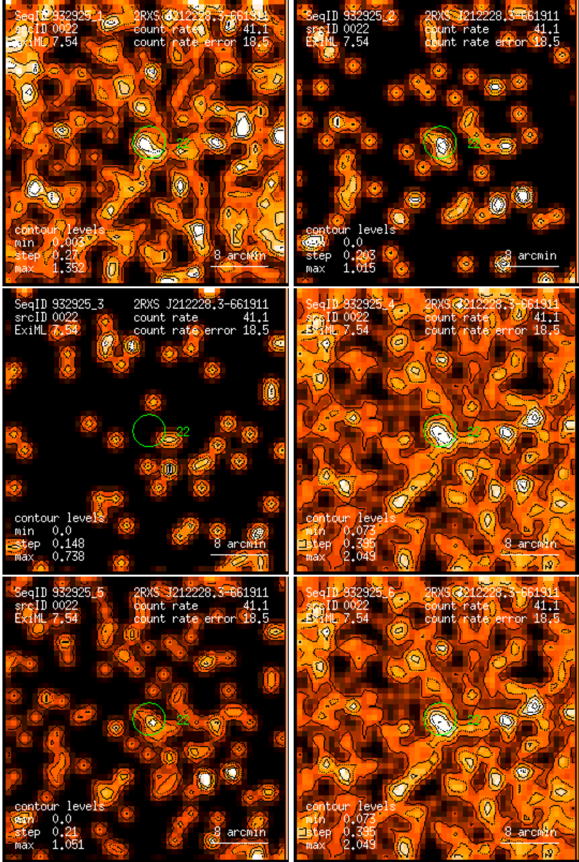
Figure 22: RASS 932925: detection 0022: band rate images, Gaussian filter: (1) PSPC channels 11 – 41, (2) 52 – 90, (3) 91 – 201, (4) 11 – 235, (5) 52 – 201, (6) 11 – 201. Broad band rates in counts/ks. Band rate contour levels in counts/ks/arcmin 2 .
