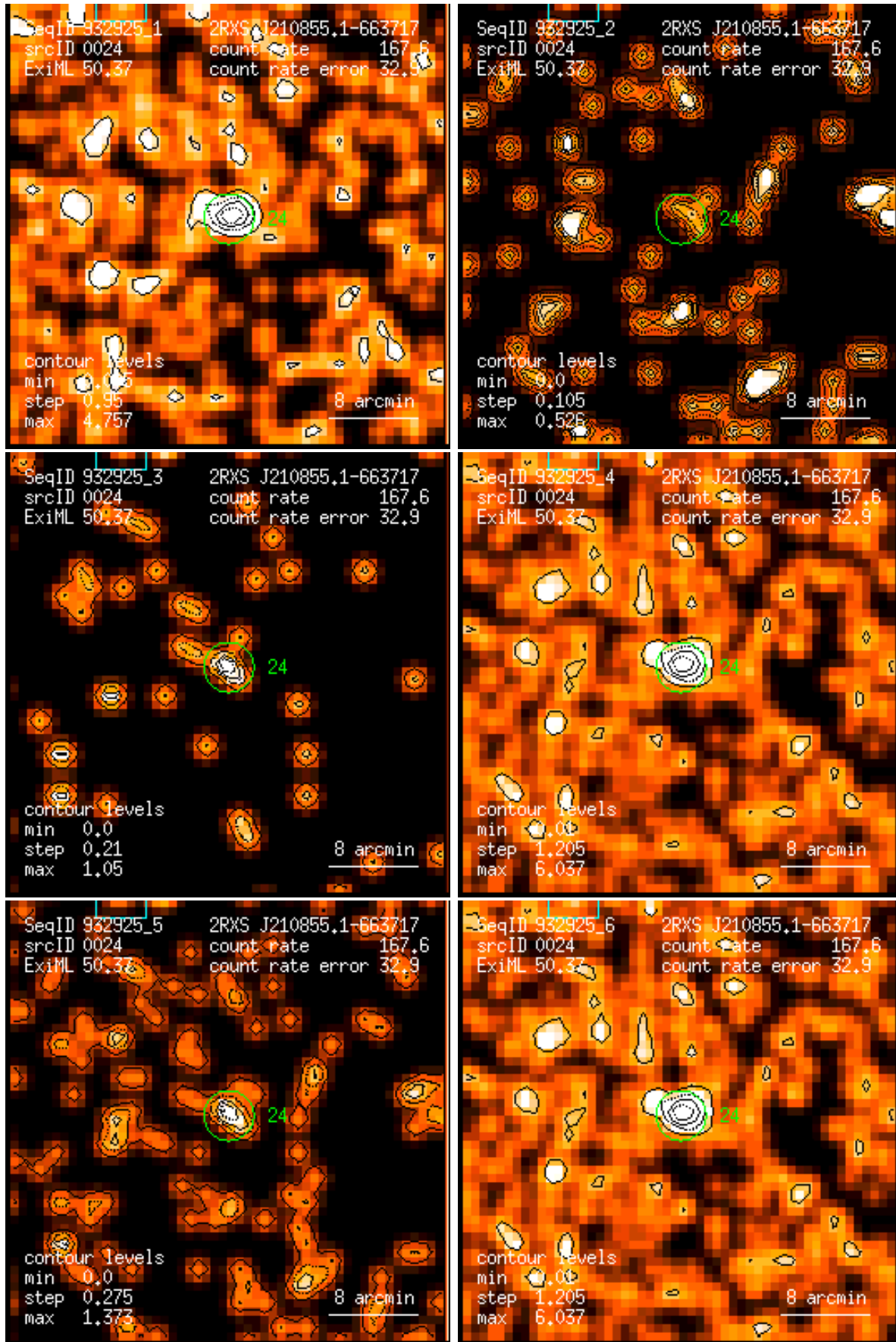
Figure 24: RASS 932925: detection 0024: band rate images, Gaussian filter: (1) PSPC channels 11 – 41, (2) 52 – 90, (3) 91 – 201, (4) 11 – 235, (5) 52 – 201, (6) 11 – 201. Broad band rates in counts/ks. Band rate contour levels in counts/ks/arcmin 2 .
