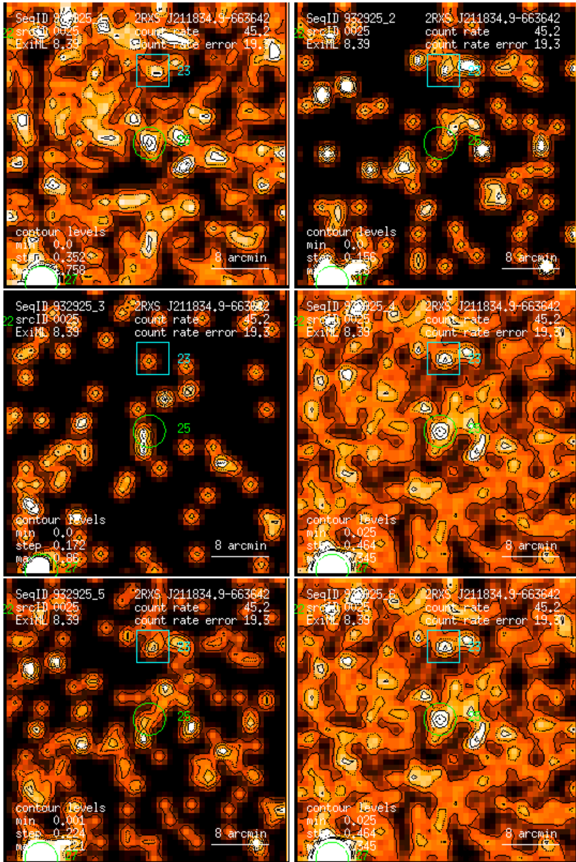
Figure 25: RASS 932925: detection 0025: band rate images, Gaussian filter: (1) PSPC channels 11 – 41, (2) 52 – 90, (3) 91 – 201, (4) 11 – 235, (5) 52 – 201, (6) 11 – 201. Broad band rates in counts/ks. Band rate contour levels in counts/ks/arcmin 2 .
