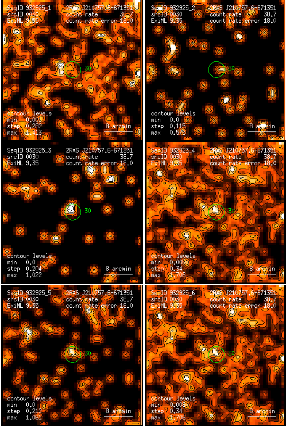
Figure 30: RASS 932925: detection 0030: band rate images, Gaussian filter: (1) PSPC channels 11 – 41, (2) 52 – 90, (3) 91 – 201, (4) 11 – 235, (5) 52 – 201, (6) 11 – 201. Broad band rates in counts/ks. Band rate contour levels in counts/ks/arcmin 2 .
