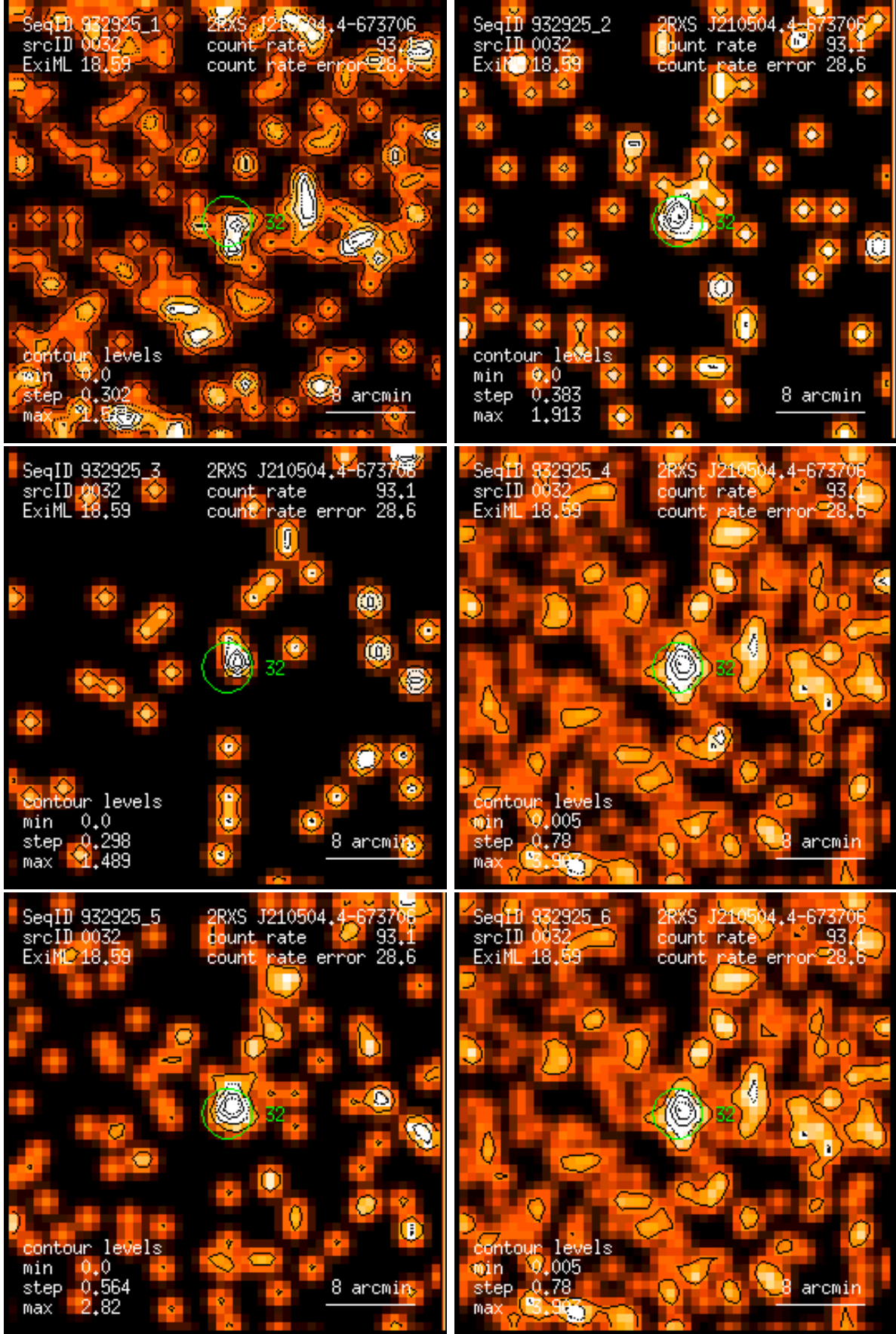
Figure 32: RASS 932925: detection 0032: band rate images, Gaussian filter: (1) PSPC channels 11 – 41, (2) 52 – 90, (3) 91 – 201, (4) 11 – 235, (5) 52 – 201, (6) 11 – 201. Broad band rates in counts/ks. Band rate contour levels in counts/ks/arcmin 2 .
