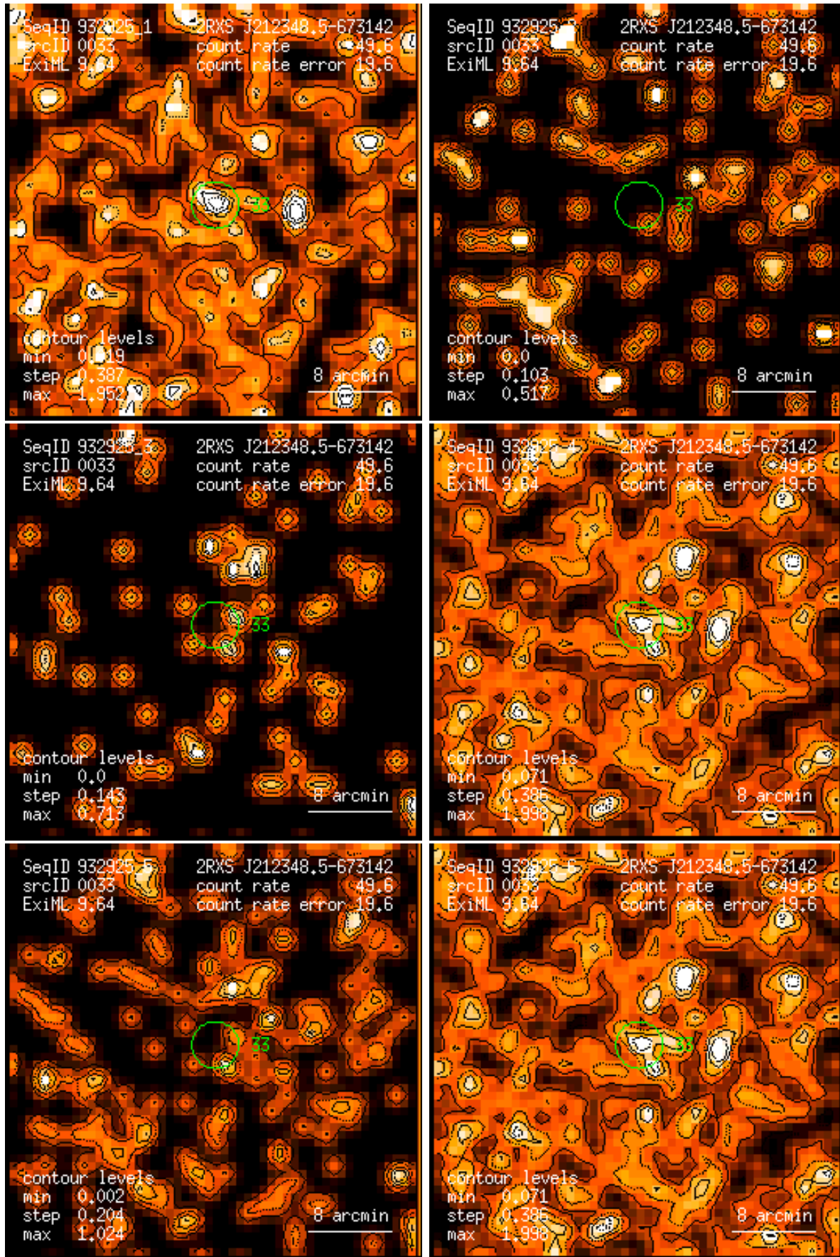
Figure 33: RASS 932925: detection 0033: band rate images, Gaussian filter: (1) PSPC channels 11 – 41, (2) 52 – 90, (3) 91 – 201, (4) 11 – 235, (5) 52 – 201, (6) 11 – 201. Broad band rates in counts/ks. Band rate contour levels in counts/ks/arcmin 2 .
