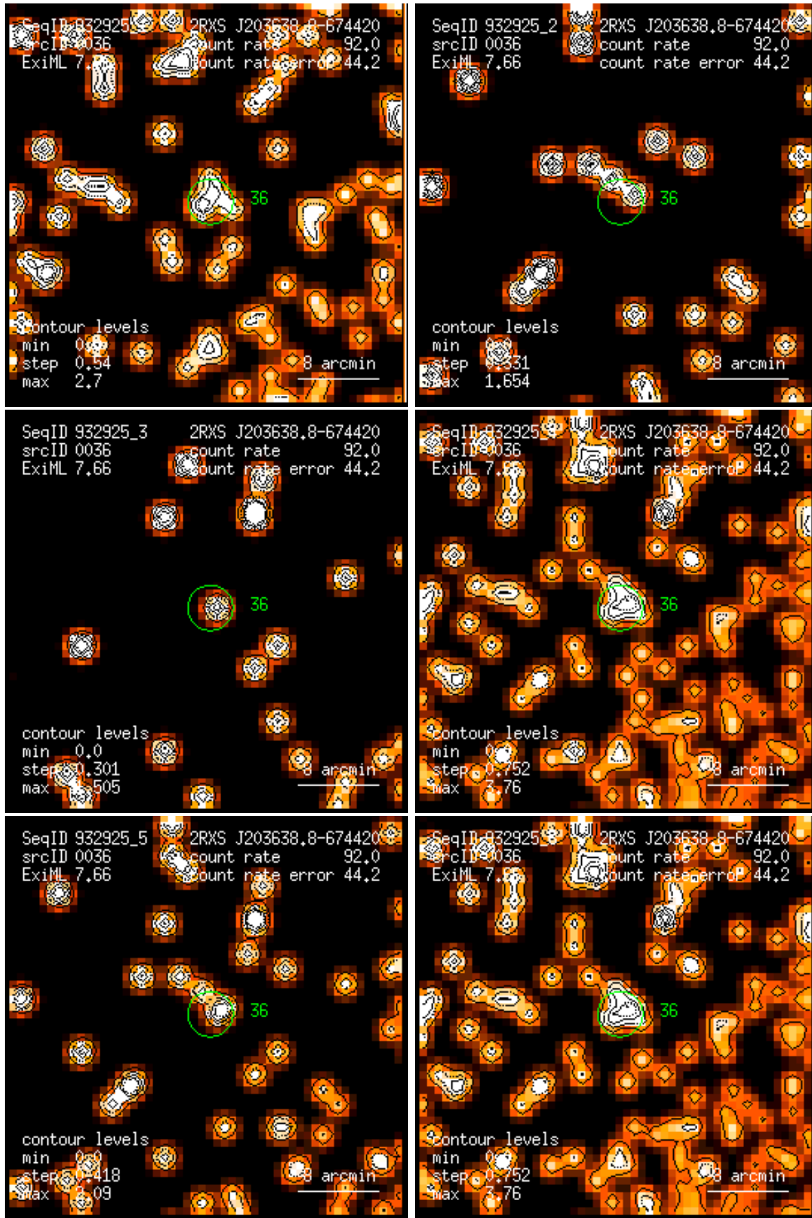
Figure 36: RASS 932925: detection 0036: band rate images, Gaussian filter: (1) PSPC channels 11 – 41, (2) 52 – 90, (3) 91 – 201, (4) 11 – 235, (5) 52 – 201, (6) 11 – 201. Broad band rates in counts/ks. Band rate contour levels in counts/ks/arcmin 2 .
