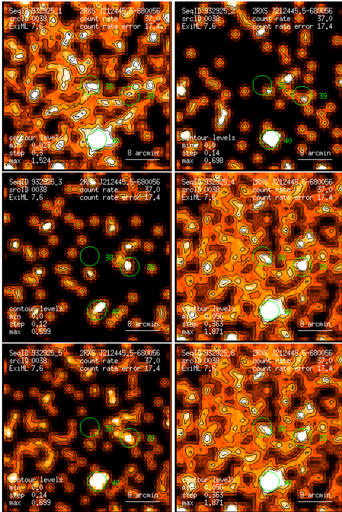
Figure 38: RASS 932925: detection 0038: band rate images, Gaussian filter: (1) PSPC channels 11 – 41, (2) 52 – 90, (3) 91 – 201, (4) 11 – 235, (5) 52 – 201, (6) 11 – 201. Broad band rates in counts/ks. Band rate contour levels in counts/ks/arcmin 2 .
