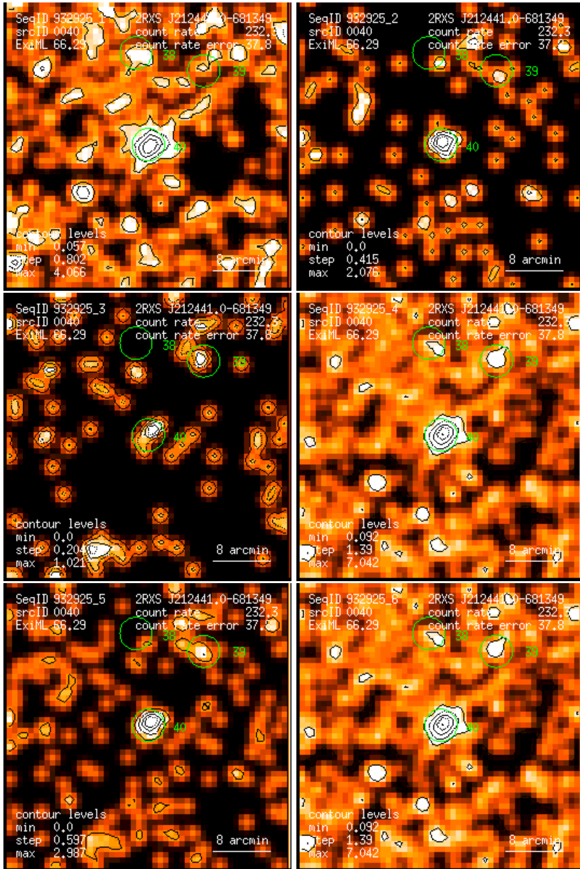
Figure 40: RASS 932925: detection 0040: band rate images, Gaussian filter: (1) PSPC channels 11 – 41, (2) 52 – 90, (3) 91 – 201, (4) 11 – 235, (5) 52 – 201, (6) 11 – 201. Broad band rates in counts/ks. Band rate contour levels in counts/ks/arcmin 2 .
