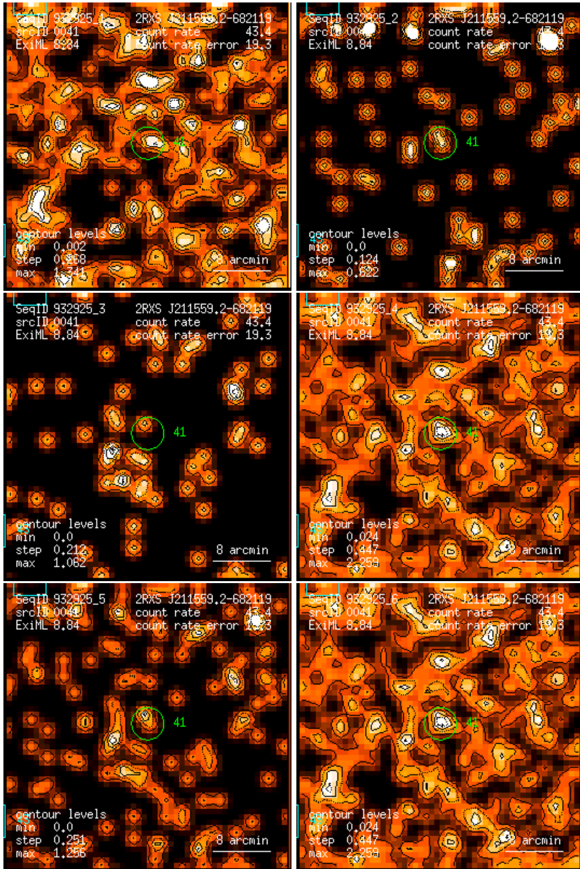
Figure 41: RASS 932925: detection 0041: band rate images, Gaussian filter: (1) PSPC channels 11 – 41, (2) 52 – 90, (3) 91 – 201, (4) 11 – 235, (5) 52 – 201, (6) 11 – 201. Broad band rates in counts/ks. Band rate contour levels in counts/ks/arcmin 2 .
