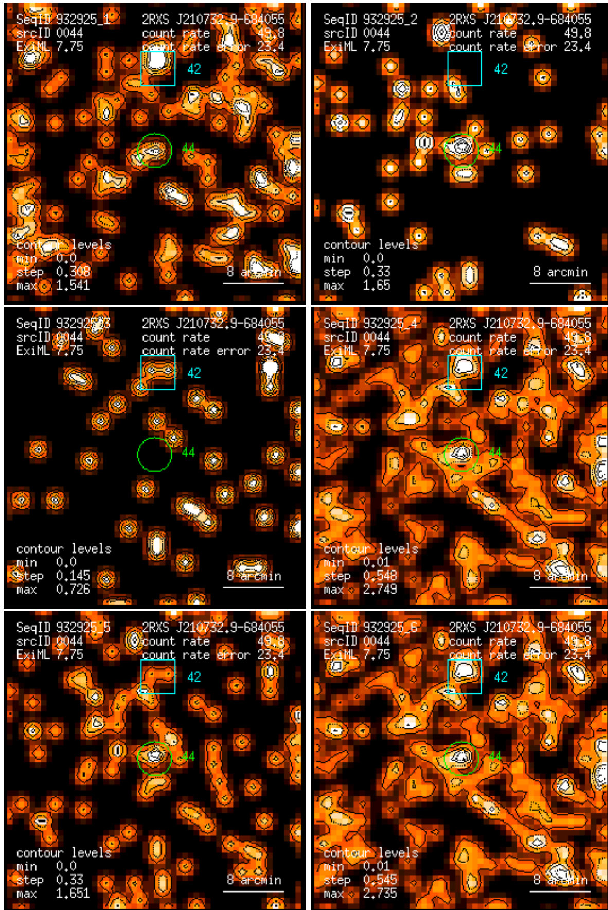
Figure 44: RASS 932925: detection 0044: band rate images, Gaussian filter: (1) PSPC channels 11 – 41, (2) 52 – 90, (3) 91 – 201, (4) 11 – 235, (5) 52 – 201, (6) 11 – 201. Broad band rates in counts/ks. Band rate contour levels in counts/ks/arcmin 2 .
