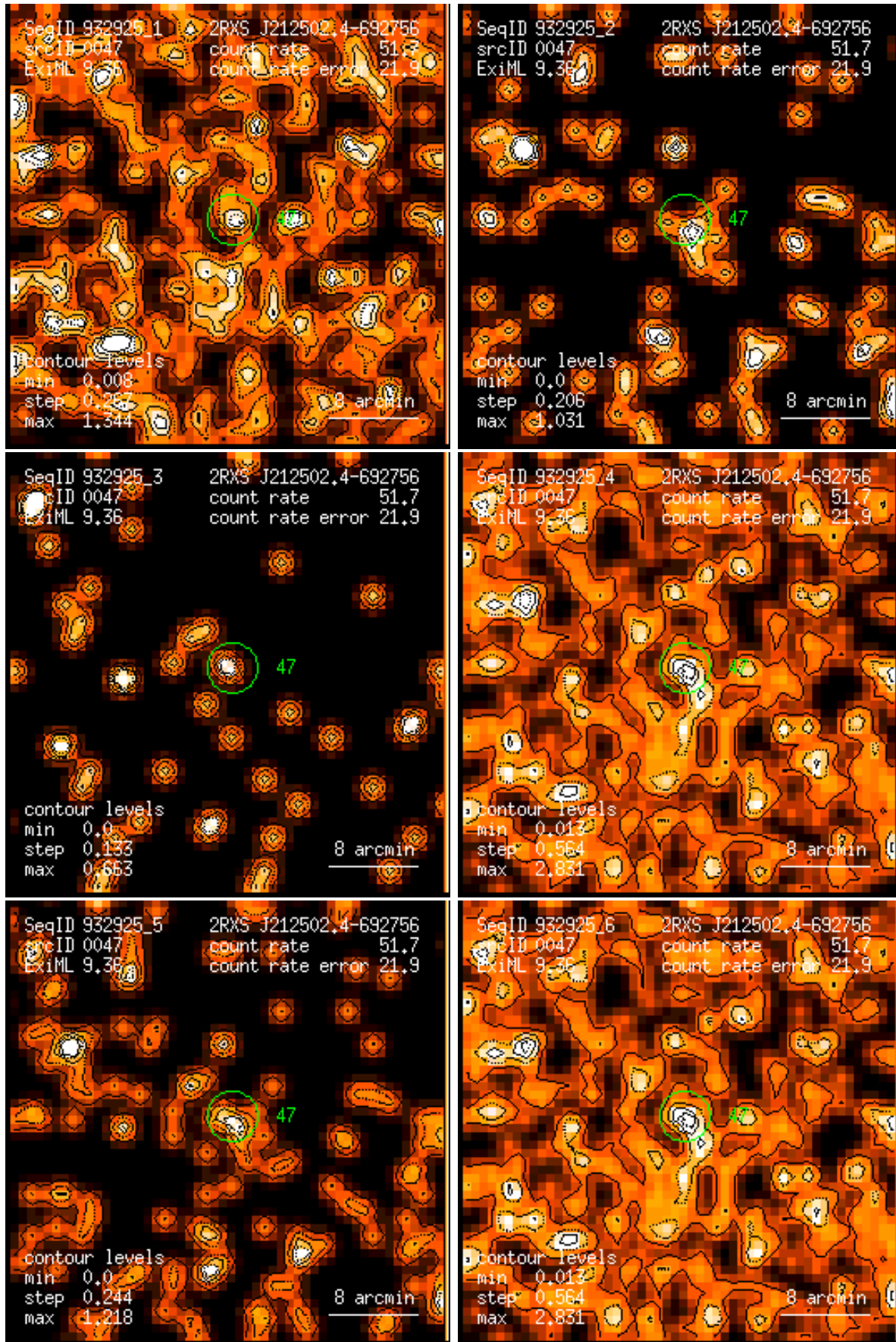
Figure 47: RASS 932925: detection 0047: band rate images, Gaussian filter: (1) PSPC channels 11 – 41, (2) 52 – 90, (3) 91 – 201, (4) 11 – 235, (5) 52 – 201, (6) 11 – 201. Broad band rates in counts/ks. Band rate contour levels in counts/ks/arcmin 2 .
