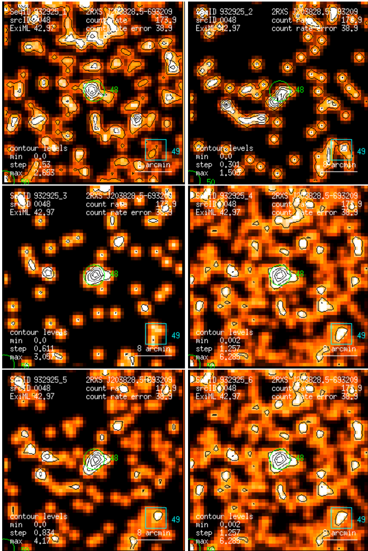
Figure 48: RASS 932925: detection 0048: band rate images, Gaussian filter: (1) PSPC channels 11 – 41, (2) 52 – 90, (3) 91 – 201, (4) 11 – 235, (5) 52 – 201, (6) 11 – 201. Broad band rates in counts/ks. Band rate contour levels in counts/ks/arcmin 2 .
