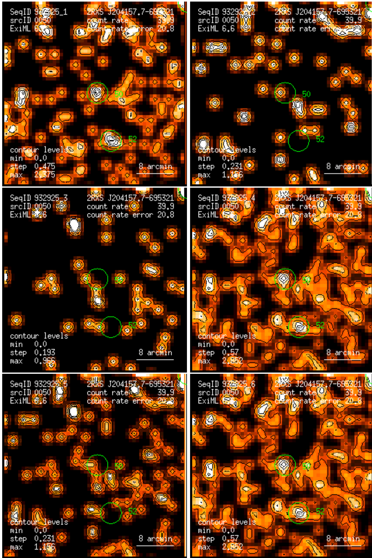
Figure 50: RASS 932925: detection 0050: band rate images, Gaussian filter: (1) PSPC channels 11 – 41, (2) 52 – 90, (3) 91 – 201, (4) 11 – 235, (5) 52 – 201, (6) 11 – 201. Broad band rates in counts/ks. Band rate contour levels in counts/ks/arcmin 2 .
