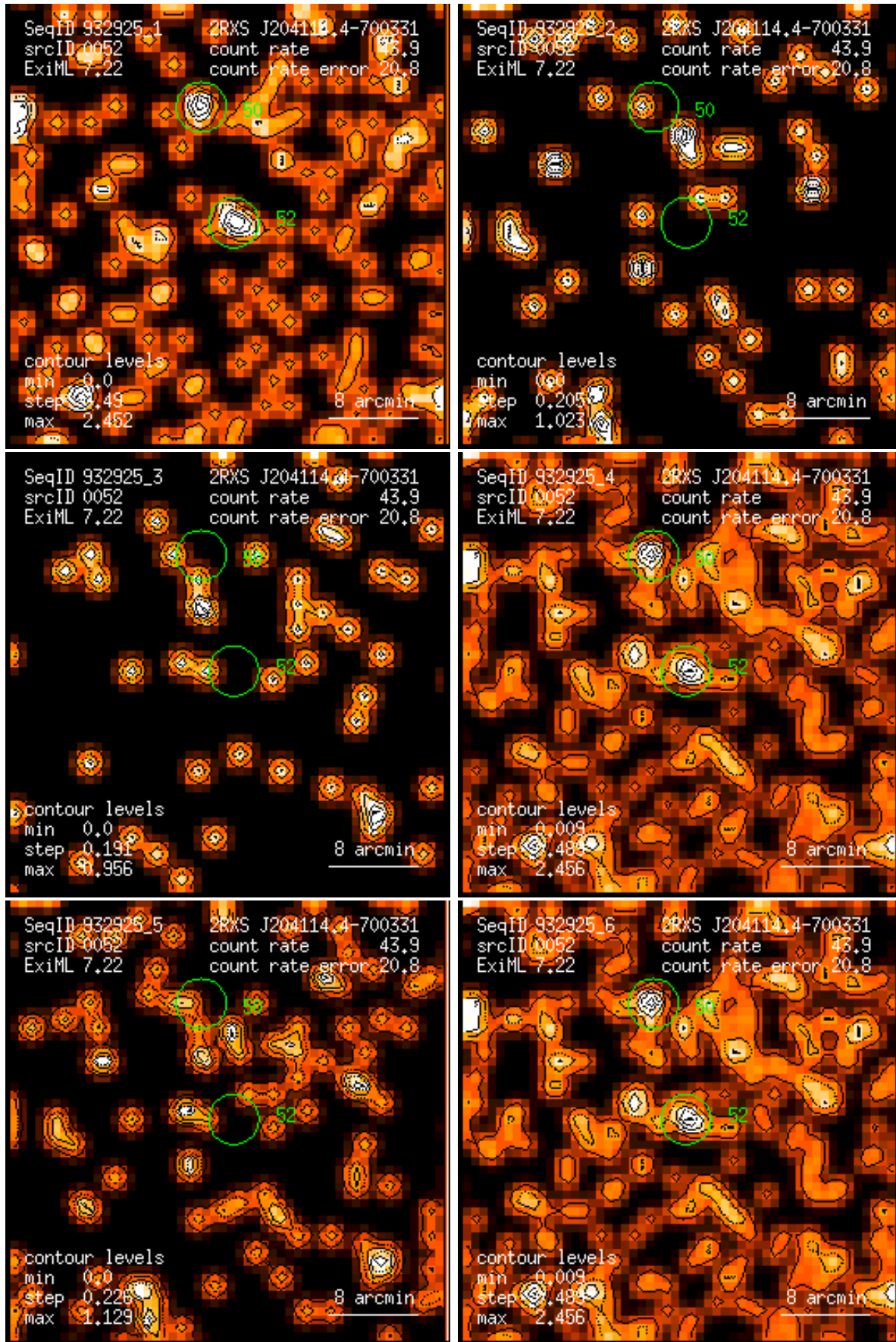
Figure 52: RASS 932925: detection 0052: band rate images, Gaussian filter: (1) PSPC channels 11 – 41, (2) 52 – 90, (3) 91 – 201, (4) 11 – 235, (5) 52 – 201, (6) 11 – 201. Broad band rates in counts/ks. Band rate contour levels in counts/ks/arcmin 2 .
