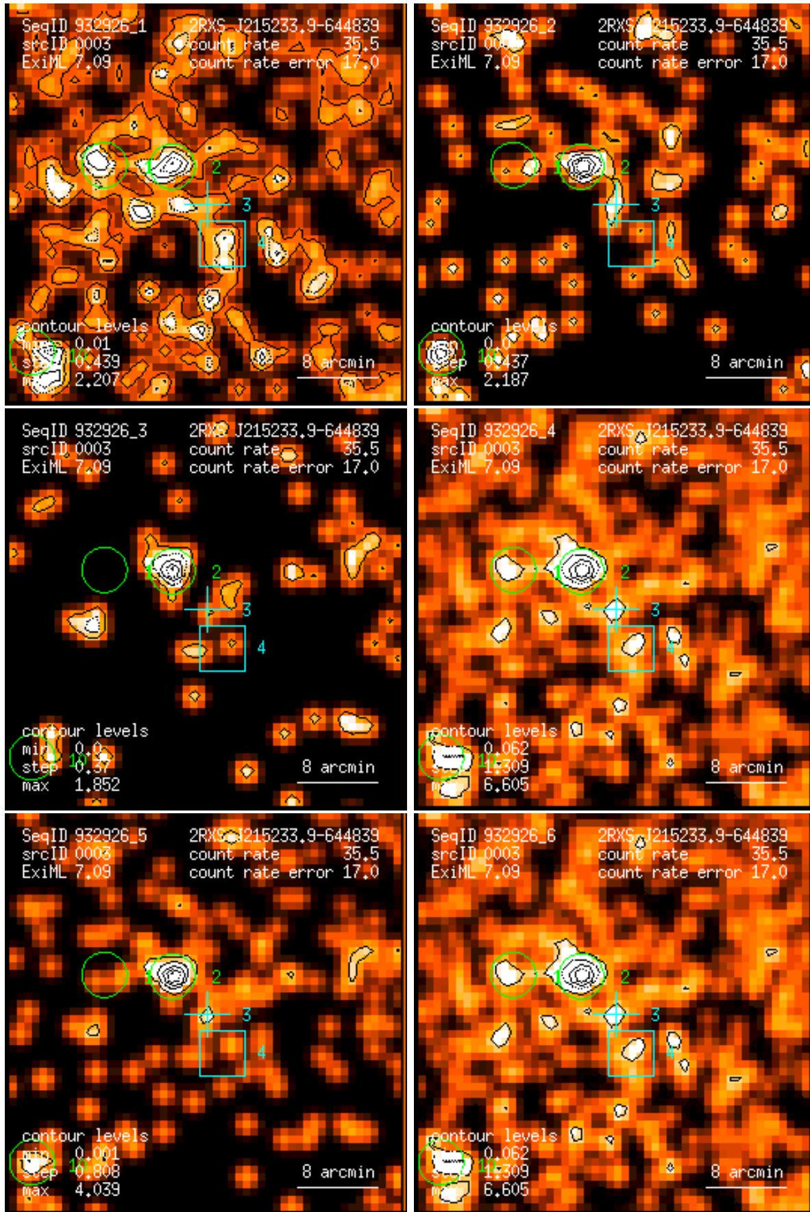
Figure 3: RASS 932926: detection 0003: band rate images, Gaussian filter: (1) PSPC channels 11 – 41, (2) 52 – 90, (3) 91 – 201, (4) 11 – 235, (5) 52 – 201, (6) 11 – 201. Broad band rates in counts/ks. Band rate contour levels in counts/ks/arcmin 2 .
