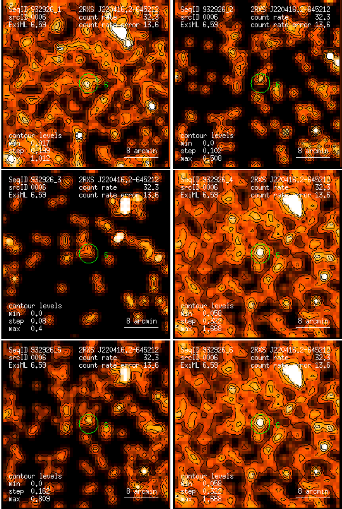
Figure 6: RASS 932926: detection 0006: band rate images, Gaussian filter: (1) PSPC channels 11 – 41, (2) 52 – 90, (3) 91 – 201, (4) 11 – 235, (5) 52 – 201, (6) 11 – 201. Broad band rates in counts/ks. Band rate contour levels in counts/ks/arcmin 2 .
